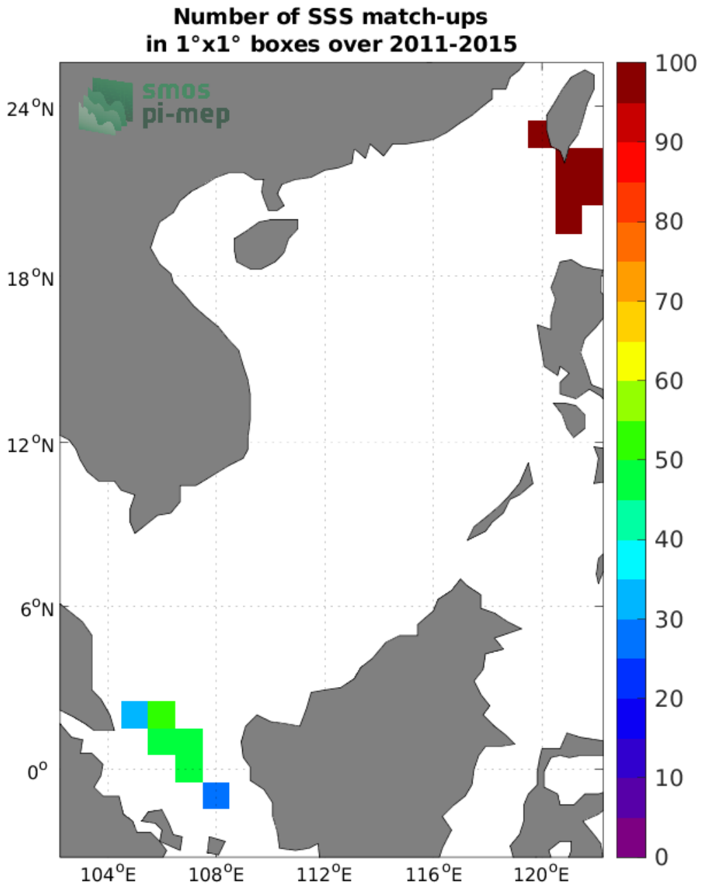
Figure 4: Number of SSS match-ups between TSG (LEGOS-DM) SSS and the Aquarius SSS L4 OI v5 - Weekly (IPRC) SSS product for the South China Sea Pi-MEP region over 1°x1° boxes and for the full satellite product period.
