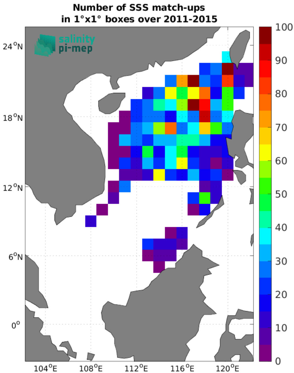
Figure 4: Number of SSS match-ups between Argo SSS and the Aquarius SSS L4 OI v5 - Weekly (IPRC) SSS product for the South China Sea Pi-MEP region over 1^{\circ} \times 1^{\circ} boxes and for the full satellite product period.
