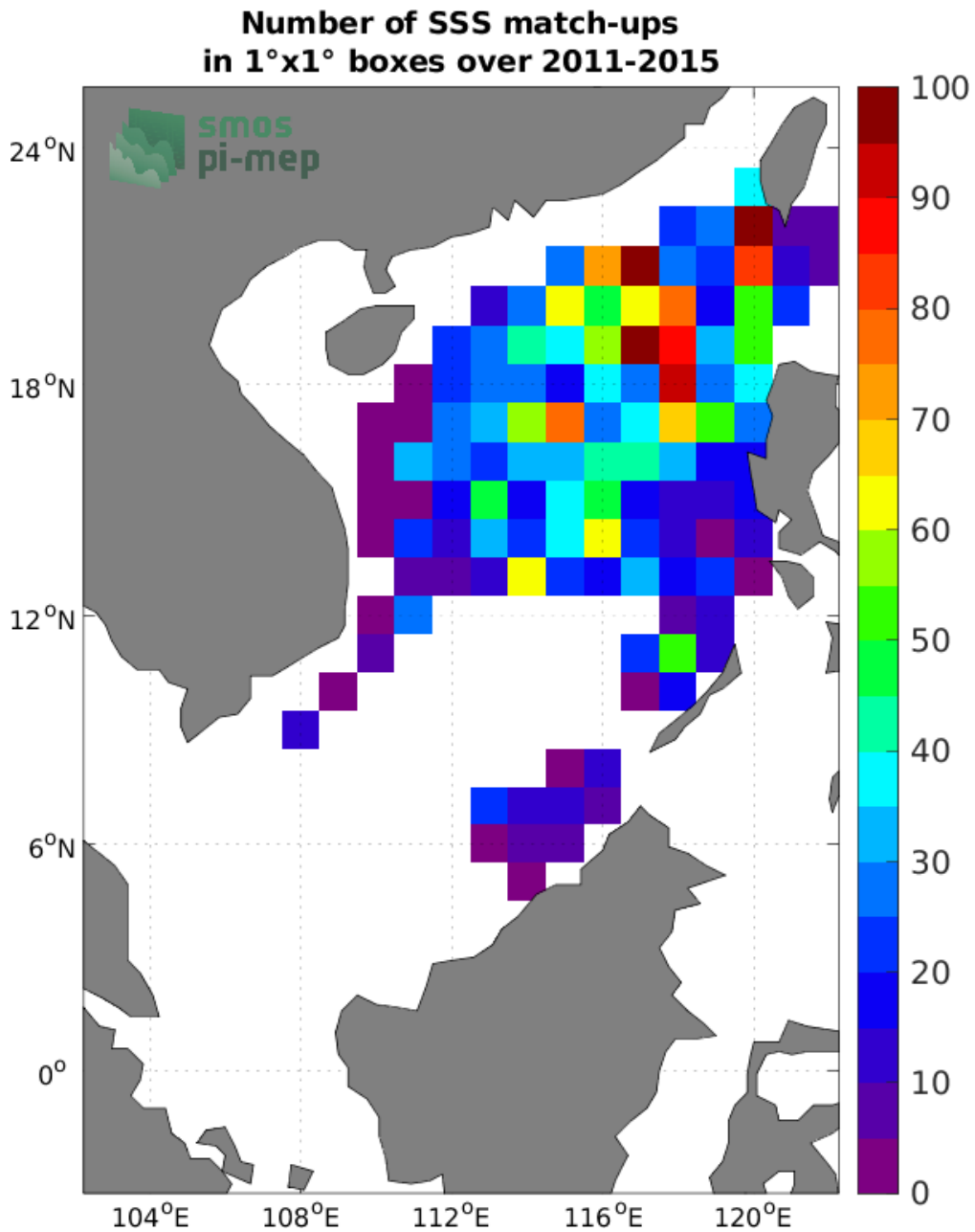
Figure 4: Number of SSS match-ups between Argo SSS and the Aquarius SSS L4 OI v5 - Weekly (IPRC) SSS product for the South China Sea Pi-MEP region over 1°x1° boxes and for the full satellite product period.
