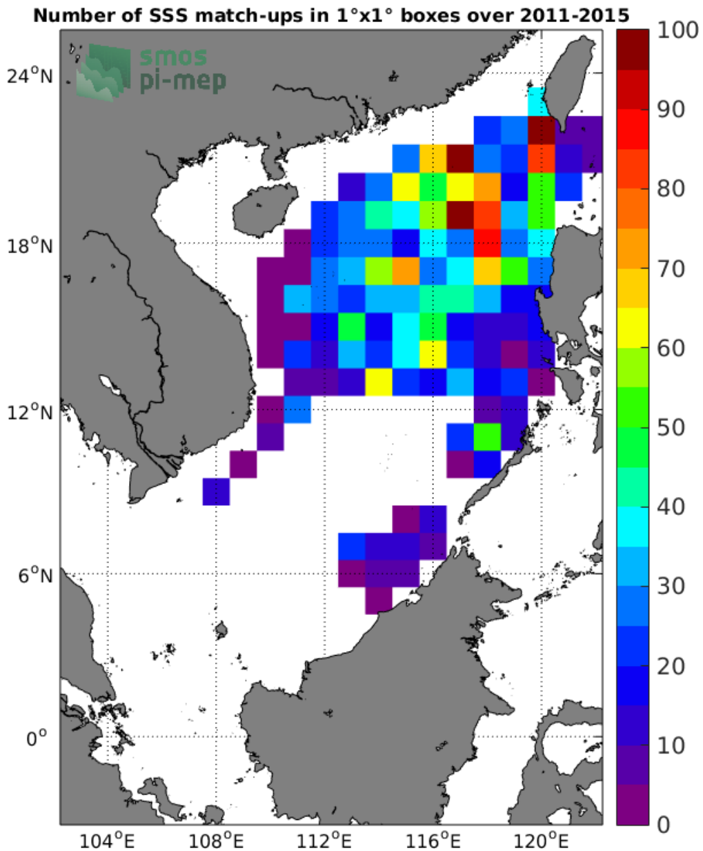
Figure 4: Number of SSS match-ups between Argo SSS and the Aquarius-L4-IPRC-V5-WEEKLY SSS product for the South China Sea Pi-MEP region over 1°x1° boxes and for the full satellite product period.
