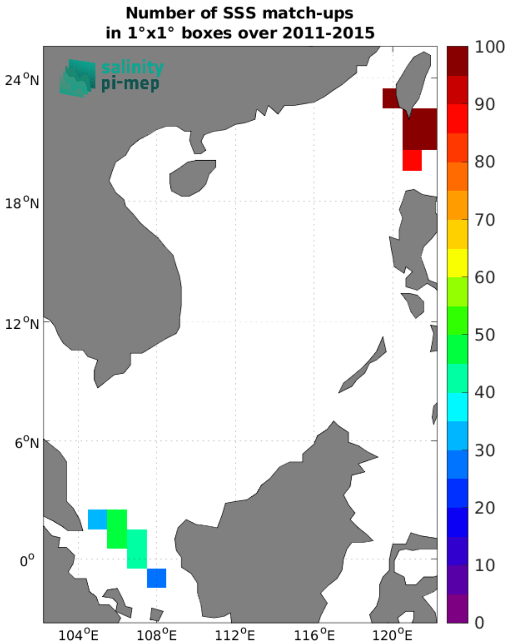
Figure 5: Number of SSS match-ups between TSG (LEGOS-DM) SSS and the Aquarius SSS L4 OI v5 - Monthly (IPRC) SSS product for the South China Sea Pi-MEP region over 1°x1° boxes and for the full satellite product period.
