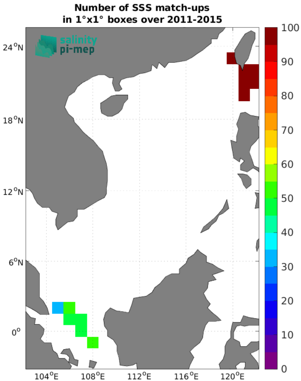
Figure 4: Number of SSS match-ups between TSG (LEGOS-DM) SSS and the Aquarius SSS L4 OI v5 - Monthly (IPRC) SSS product for the South China Sea Pi-MEP region over 1^{\circ} \times 1^{\circ} boxes and for the full satellite product period.
