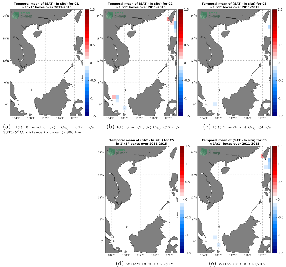
Figure 12: Temporal mean gridded over spatial boxes of size 1^\circ \times 1^\circ of \Delta SSS (Aquarius-L4-IPRC-V5-MONTHLY - TSG-LEGOS-DM) for 5 different subdatasets corresponding to:RR=0 mm/h, 3 < U_{10} < 12 m/s, SST>5°C, distance to coast > 800 km (a), RR=0 mm/h, 3 < U_{10} < 12 m/s (b), RR>1mm/h and U_{10} < 4 m/s (c), WOA2013 SSS Std<0.2 (d), WOA2013 SSS Std>0.2 (e).
