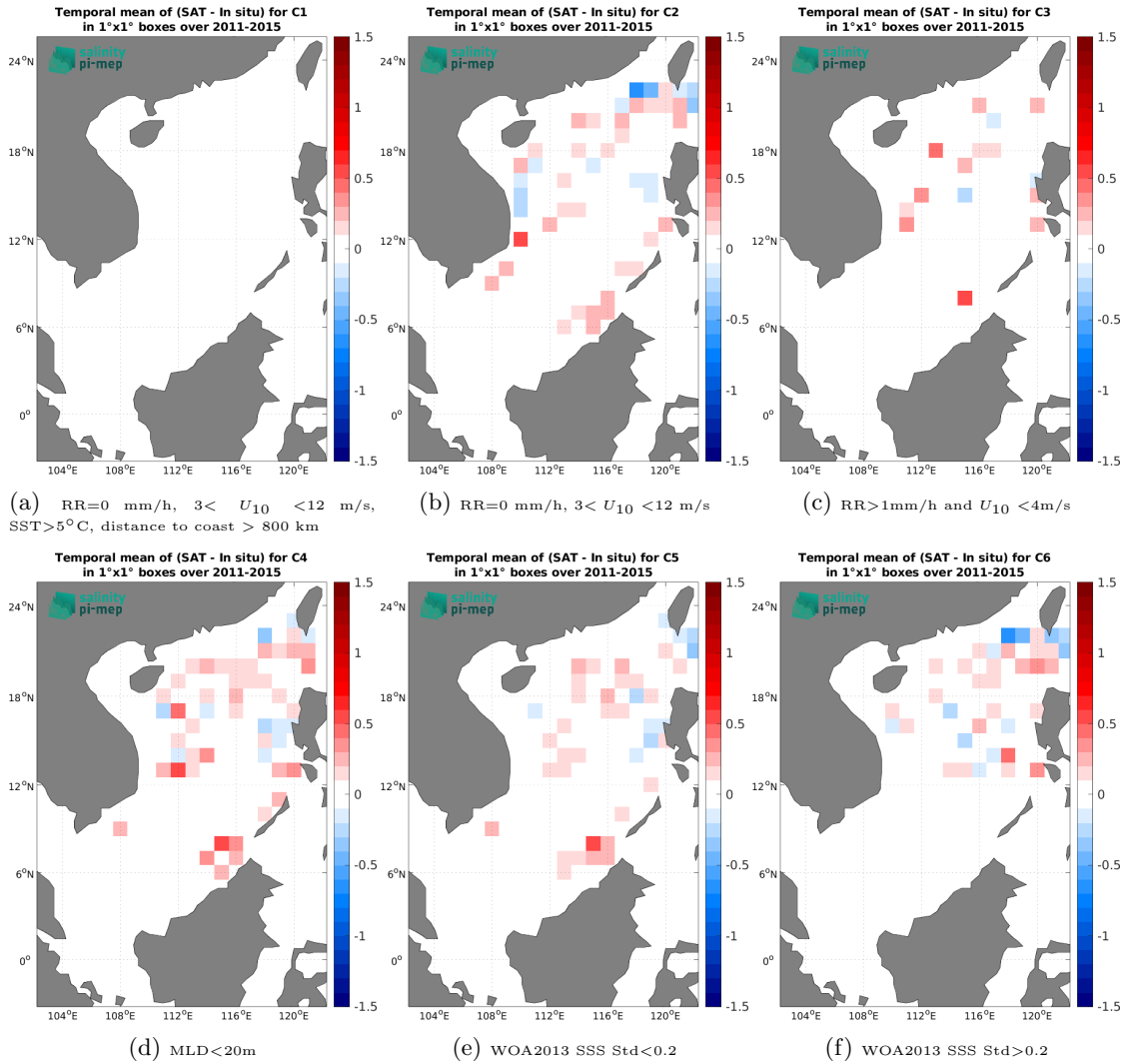
Figure 14: Temporal mean gridded over spatial boxes of size 1^\circ \times 1^\circ of \Delta\text{SSS} (Aquarius SSS L4 OI v5 - Monthly (IPRC) - Argo) for 6 different subdatasets corresponding to: RR=0 mm/h, 3 < U_{10} < 12 m/s, SST > 5^\circ\text{C} , distance to coast > 800 km (a), RR=0 mm/h, 3 < U_{10} < 12 m/s (b), RR > 1\text{mm/h} and U_{10} < 4\text{m/s} (c), MLD < 20\text{m} (d), WOA2013 SSS Std < 0.2 (e), WOA2013 SSS Std > 0.2 (f).
