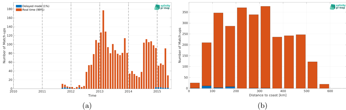
Figure 2: Number of match-ups between Argo and Aquarius SSS L4 OI v5 - Monthly (IPRC) SSS as a function of time (a) and as function of the distance to coast (b) over the South China Sea Pi-MEP region and for the full satellite product period.
