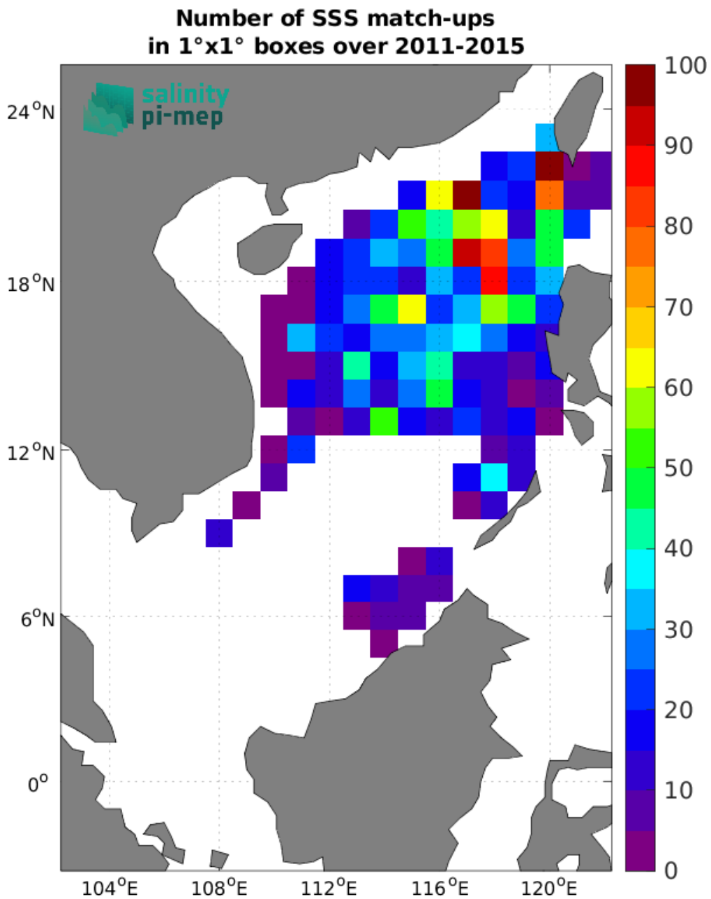
Figure 5: Number of SSS match-ups between Argo SSS and the Aquarius SSS L4 OI v5 - Monthly (IPRC) SSS product for the South China Sea Pi-MEP region over 1^\circ \times 1^\circ boxes and for the full satellite product period.
