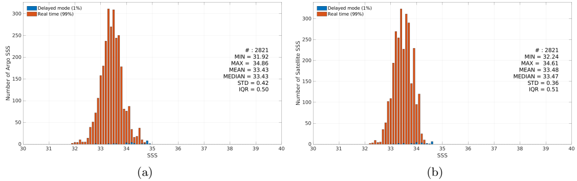
Figure 3: Histograms of SSS from Argo (a) and Aquarius SSS L4 OI v5 - Monthly (IPRC) (b) considering all match-up pairs per bins of 0.1 over the South China Sea Pi-MEP region and for the full satellite product period.
