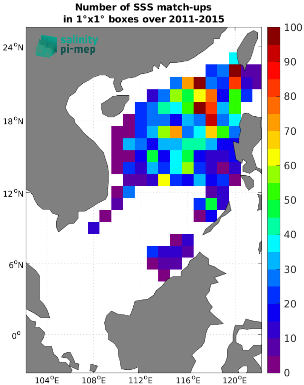
Figure 4: Number of SSS match-ups between Argo SSS and the Aquarius SSS L4 OI v5 - Monthly (IPRC) SSS product for the South China Sea Pi-MEP region over 1^\circ \times 1^\circ boxes and for the full satellite product period.
