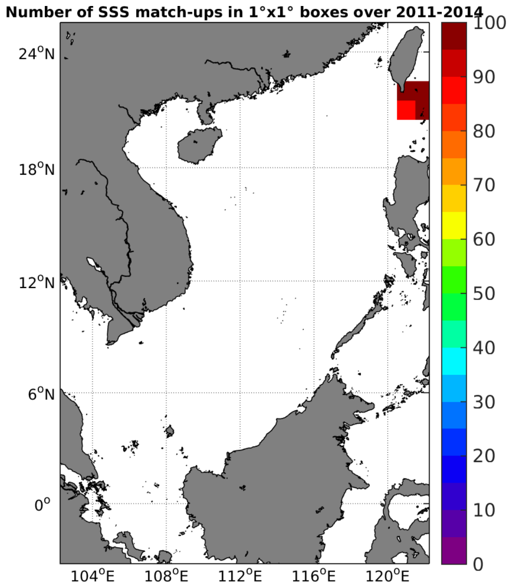
Figure 4: Number of SSS match-ups between TSG-LEGOS-DM SSS and the Aquarius-L4-IPRC-V4-MONTHLY SSS product for the South China Sea Pi-MEP region over 1°x1° boxes and for the full satellite product period.
