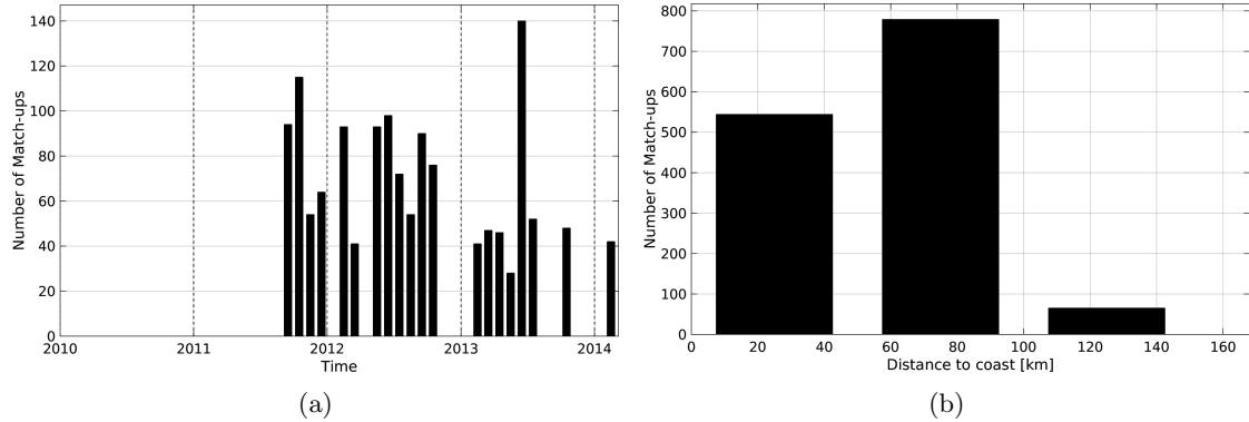
Figure 1: Number of match-ups between TSG-LEGOS-DM and Aquarius-L4-IPRC-V4-MONTHLY SSS as a function of time (a) and as function of the distance to coast (b) over the South China Sea Pi-MEP region and for the full satellite product period.
