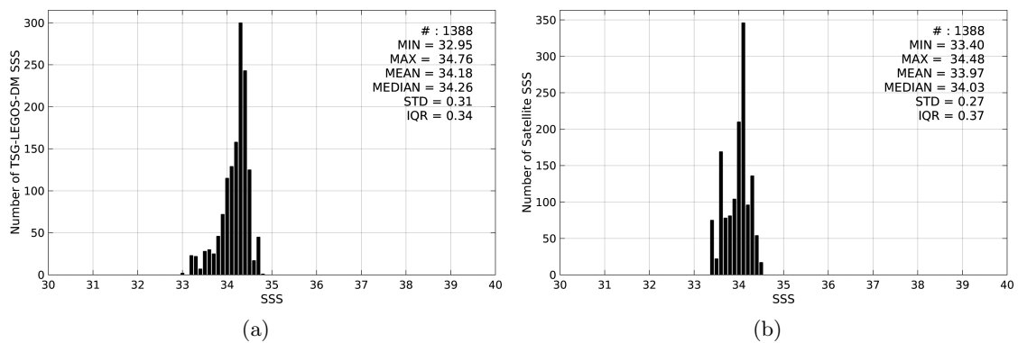
Figure 2: Histograms of SSS from TSG-LEGOS-DM (a) and Aquarius-L4-IPRC-V4-MONTHLY (b) considering all match-up pairs per bins of 0.1 over the South China Sea Pi-MEP region and for the full satellite product period.
