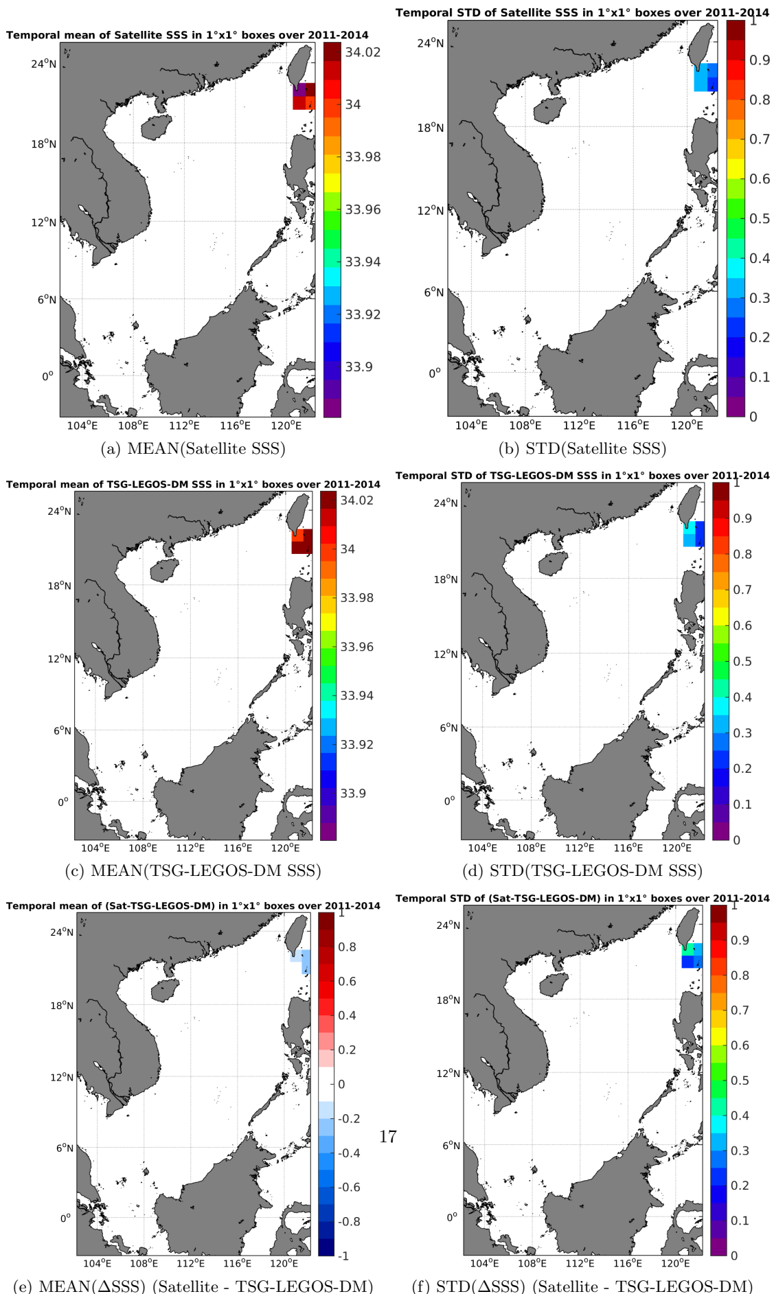
Figure 6: Temporal mean (left) and STD (right) of SSS from Aquarius-L4-IPRC-V4-MONTHLY (top), TSG-LEGOS-DM (middle), and of \Delta SSS (Satellite - TSG-LEGOS-DM). Only match-up pairs are used to generate these maps.
