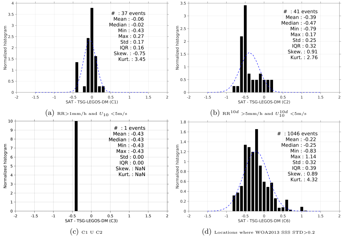
Figure 13: Normalized histogram of \Delta\text{SSS} (Aquarius-L4-IPRC-V4-MONTHLY - TSG-LEGOS-DM) for 6 different subdatasets corresponding to: RR>1mm/h and U_{10} < 5\text{m/s} (a), RR^{10d} > 5\text{mm/h} and U_{10}^{10d} < 5\text{m/s} (b), C1 U C2 (c), Locations where WOA2013 SSS STD>0.2 (d).
