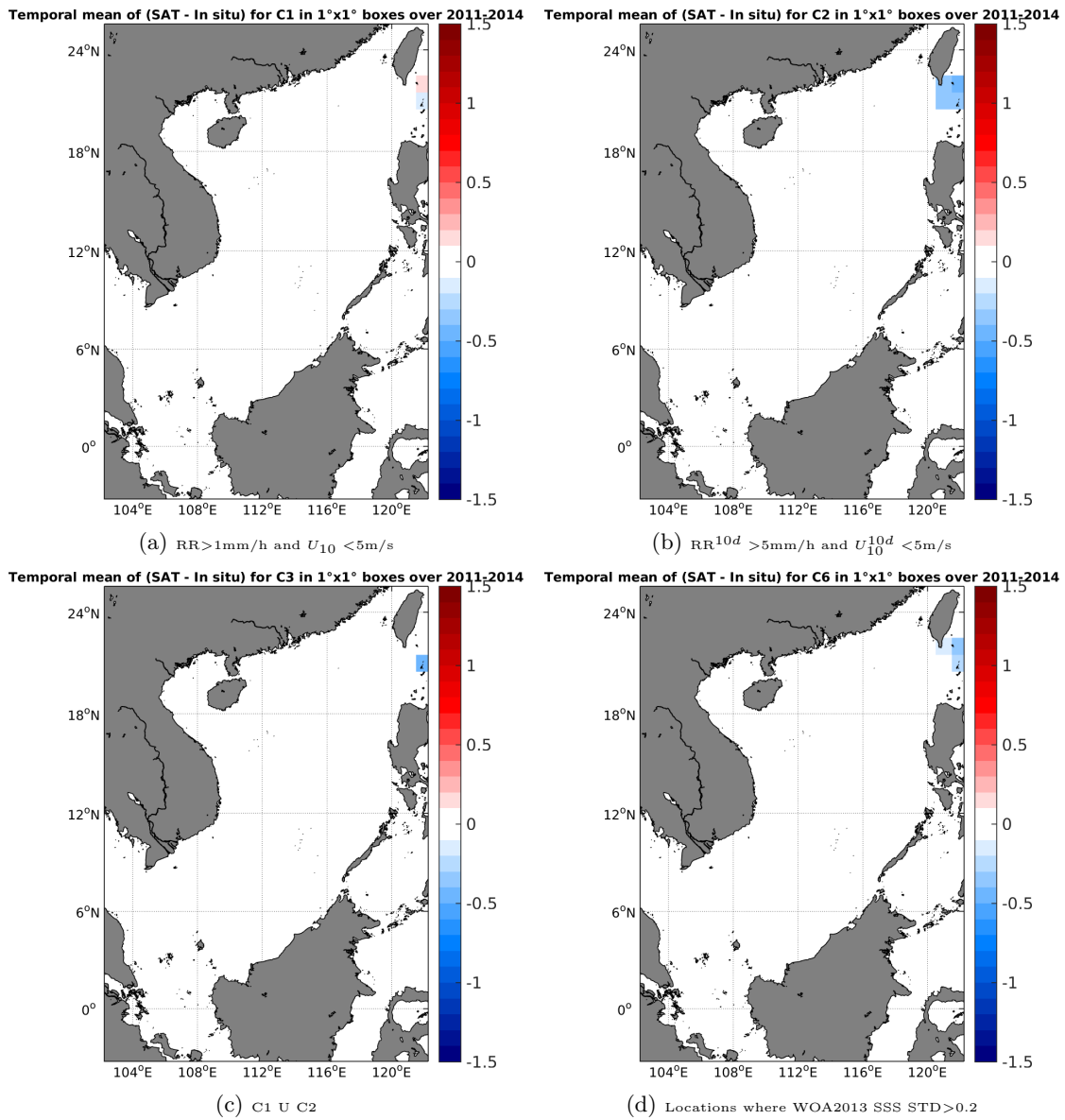
Figure 12: Temporal mean gridded over spatial boxes of size 1°x1° of \Delta\text{SSS} (Aquarius-L4-IPRC-V4-MONTHLY - TSG-LEGOS-DM) for 4 different subdatasets corresponding to: RR > 1\text{mm/h} and U_{10} < 5\text{m/s} (a), RR^{10d} > 5\text{mm/h} and U_{10}^{10d} < 5\text{m/s} (b), C1 U C2 (c), Locations where WOA2013 SSS STD > 0.2 (d).
