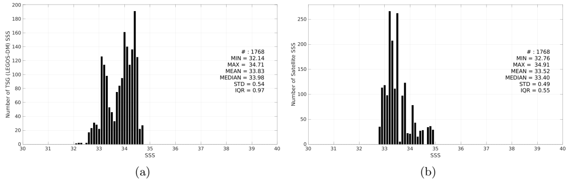
Figure 3: Histograms of SSS from TSG (LEGOS-DM) (a) and Aquarius SSS L3 OR v5 - 7-Day running (NASA-GSFC) (b) considering all match-up pairs per bins of 0.1 over the South China Sea Pi-MEP region and for the full satellite product period.
