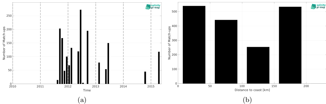
Figure 2: Number of match-ups between TSG (LEGOS-DM) and Aquarius SSS L3 OR v5 - 7-Day running (NASA-GSFC) SSS as a function of time (a) and as function of the distance to coast (b) over the South China Sea Pi-MEP region and for the full satellite product period.
