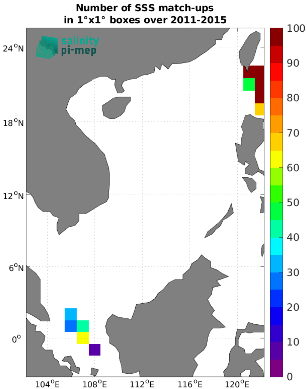
Figure 5: Number of SSS match-ups between TSG (LEGOS-DM) SSS and the Aquarius SSS L3 OR v5 - 7-Day running (NASA-GSFC) SSS product for the South China Sea Pi-MEP region over 1°×1° boxes and for the full satellite product period.
