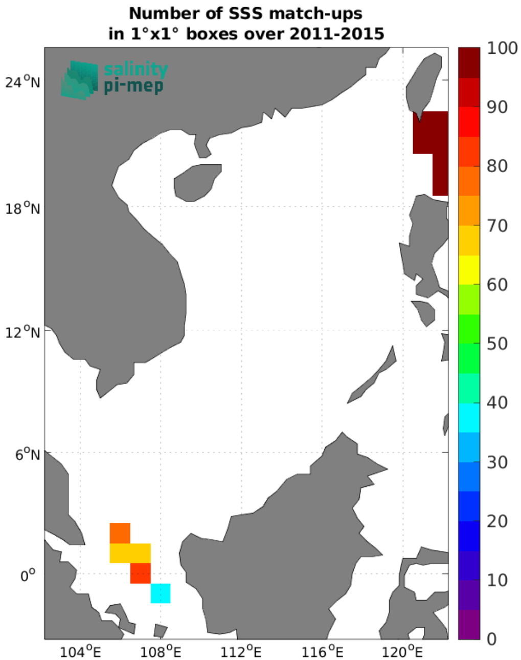
Figure 4: Number of SSS match-ups between TSG (LEGOS-DM) SSS and the Aquarius SSS L3 OR v5 - 7-Day running (NASA-GSFC) SSS product for the South China Sea Pi-MEP region over 1^\circ \times 1^\circ boxes and for the full satellite product period.
