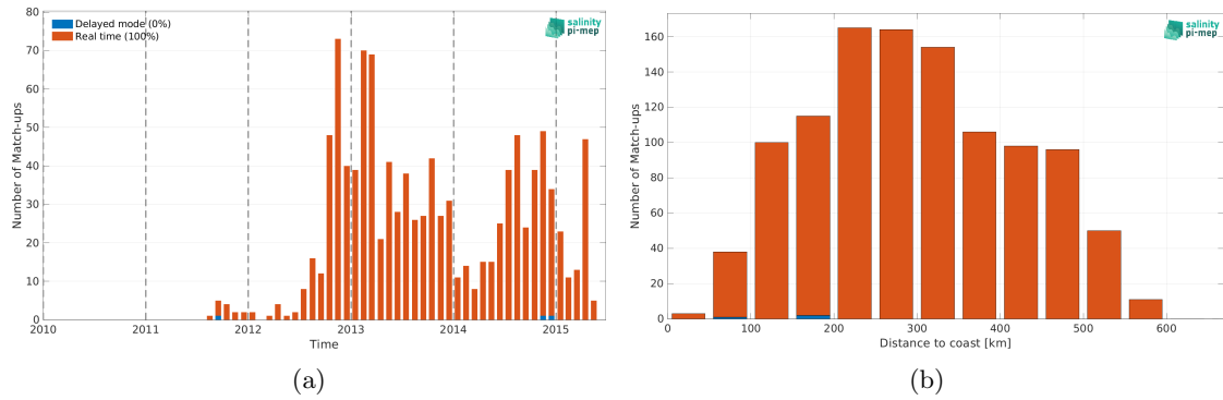
Figure 2: Number of match-ups between Argo and Aquarius SSS L3 OR v5 - 7-Day running (NASA-GSFC) SSS as a function of time (a) and as function of the distance to coast (b) over the South China Sea Pi-MEP region and for the full satellite product period.
