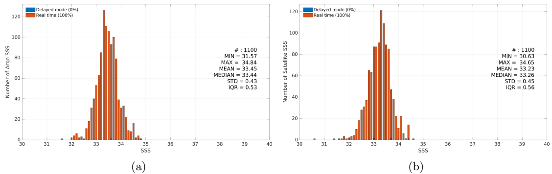
Figure 3: Histograms of SSS from Argo (a) and Aquarius SSS L3 OR v5 - 7-Day running (NASA-GSFC) (b) considering all match-up pairs per bins of 0.1 over the South China Sea Pi-MEP region and for the full satellite product period.
