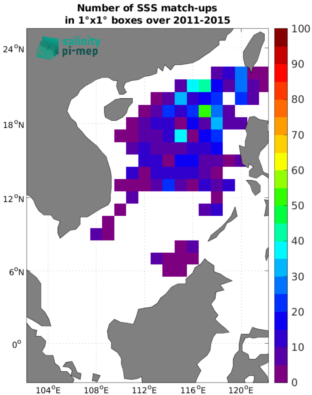
Figure 5: Number of SSS match-ups between Argo SSS and the Aquarius SSS L3 OR v5 - 7-Day running (NASA-GSFC) SSS product for the South China Sea Pi-MEP region over 1°x1° boxes and for the full satellite product period.
