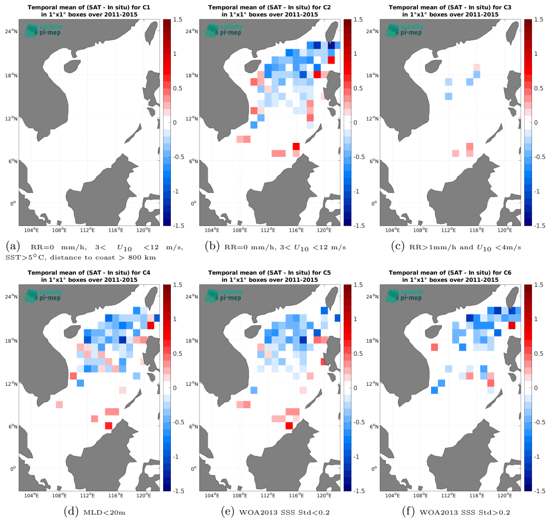
Figure 14: Temporal mean gridded over spatial boxes of size 1^\circ \times 1^\circ of \Delta\text{SSS} (Aquarius SSS L3 OR v5 - 7-Day running (NASA-GSFC) - Argo) for 6 different subdatasets corresponding to: RR=0 mm/h, 3 < U_{10} < 12 m/s, SST > 5^\circ\text{C} , distance to coast > 800 km (a), RR=0 mm/h, 3 < U_{10} < 12 m/s (b), RR > 1 mm/h and U_{10} < 4 m/s (c), MLD < 20 m (d), WOA2013 SSS Std < 0.2 (e), WOA2013 SSS Std > 0.2 (f).
