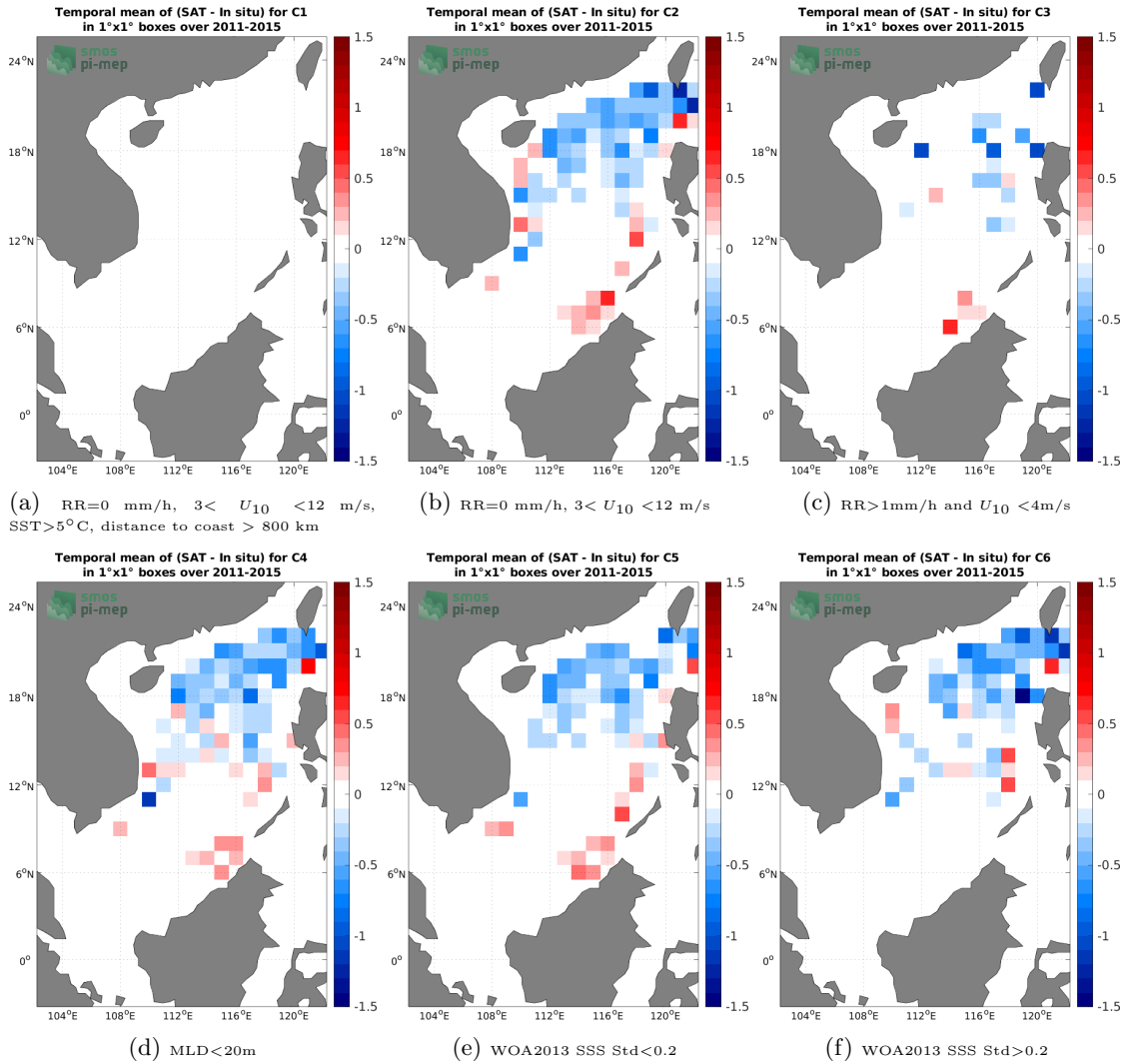
Figure 12: Temporal mean gridded over spatial boxes of size 1^\circ \times 1^\circ of \Delta\text{SSS} (Aquarius SSS L3 OR v5 - 7-Day running (NASA-GSFC) - Argo) for 6 different subdatasets corresponding to: RR=0 mm/h, 3 < U_{10} < 12 m/s, SST > 5^\circ\text{C} , distance to coast > 800 km (a), RR=0 mm/h, 3 < U_{10} < 12 m/s (b), RR > 1 mm/h and U_{10} < 4 m/s (c), MLD < 20 m (d), WOA2013 SSS Std < 0.2 (e), WOA2013 SSS Std > 0.2 (f).
