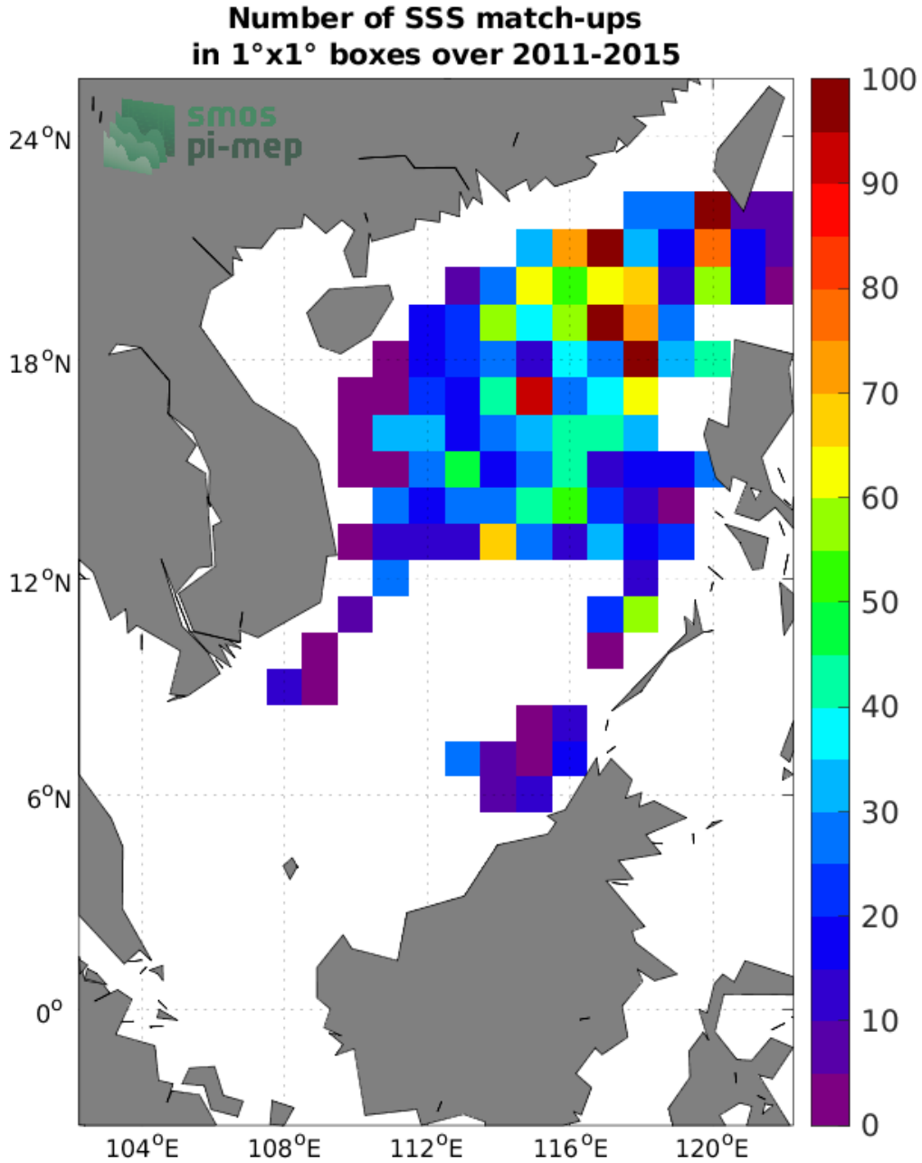
Figure 4: Number of SSS match-ups between Argo SSS and the Aquarius SSS L3 OR v5 - 7-Day running (NASA-GSFC) SSS product for the South China Sea Pi-MEP region over 1^\circ \times 1^\circ boxes and for the full satellite product period.
