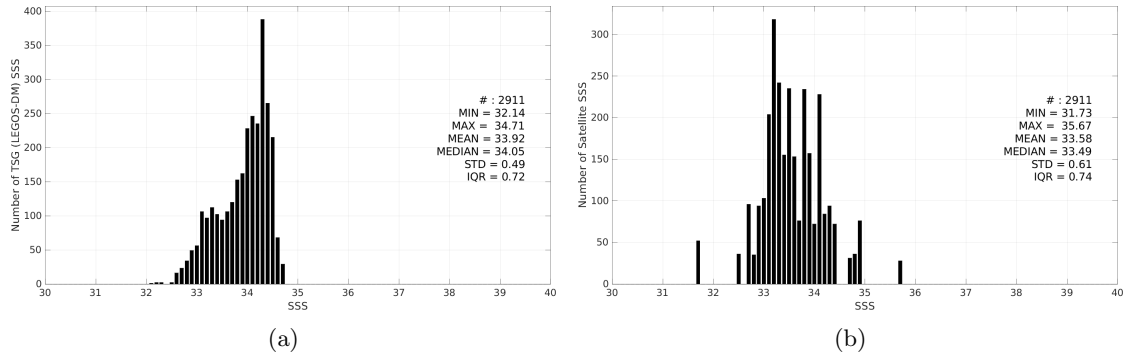
Figure 3: Histograms of SSS from TSG (LEGOS-DM) (a) and Aquarius SSS L3 OR v5 - 7-Day running - Rain mask (NASA-GSFC) (b) considering all match-up pairs per bins of 0.1 over the South China Sea Pi-MEP region and for the full satellite product period.
