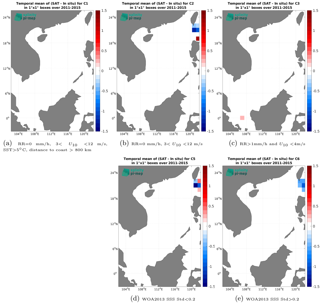
Figure 14: Temporal mean gridded over spatial boxes of size 1^\circ \times 1^\circ of \Delta\text{SSS} (Aquarius SSS L3 OR v5 - 7-Day running - Rain mask (NASA-GSFC) - TSG (LEGOS-DM)) for 5 different subdatasets corresponding to: RR=0 mm/h, 3 < U_{10} < 12 m/s, SST > 5^\circ\text{C} , distance to coast > 800 km (a), RR=0 mm/h, 3 < U_{10} < 12 m/s (b), RR > 1 mm/h and U_{10} < 4 m/s (c), WOA2013 SSS Std < 0.2 (d), WOA2013 SSS Std > 0.2 (e).
