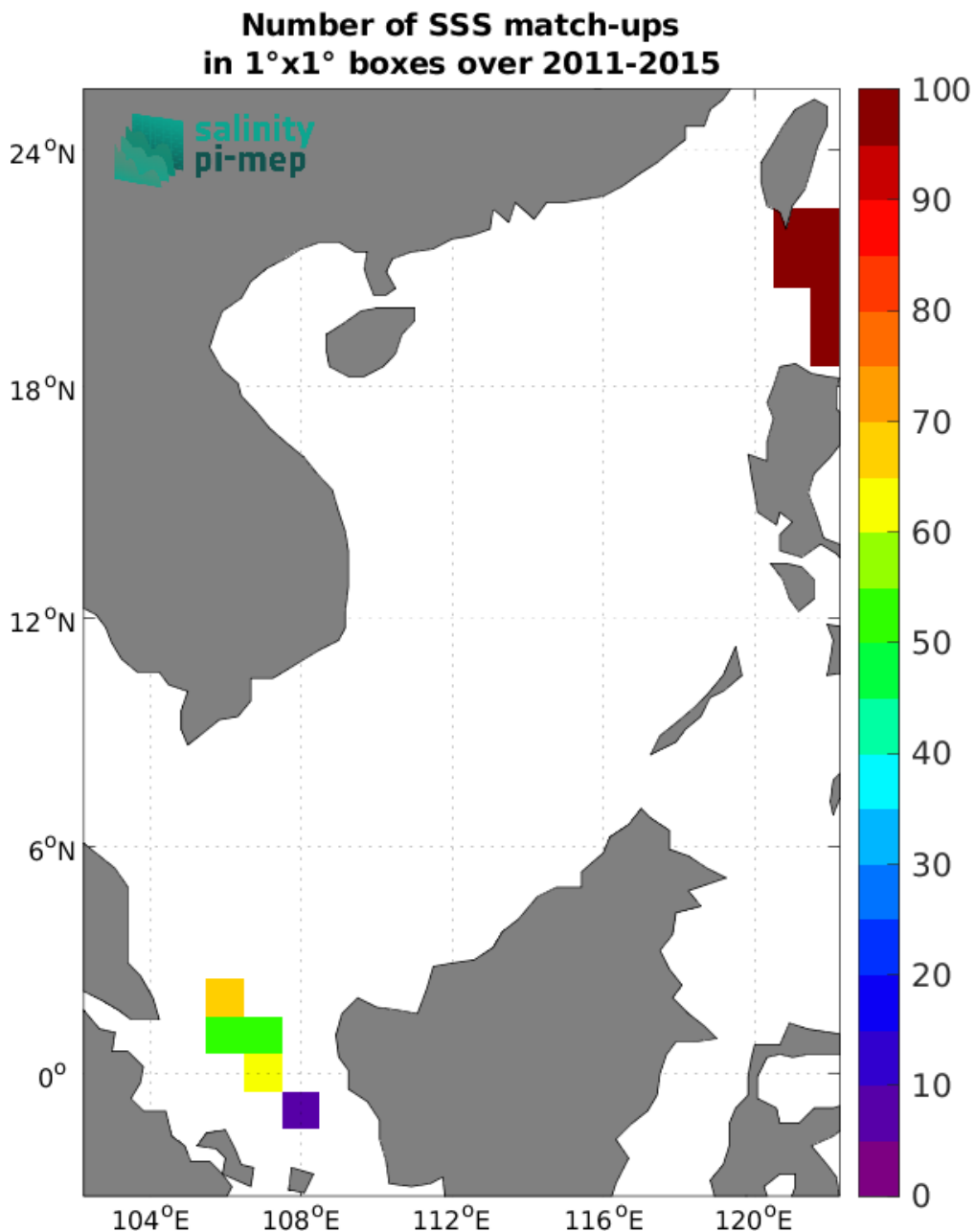
Figure 5: Number of SSS match-ups between TSG (LEGOS-DM) SSS and the Aquarius SSS L3 OR v5 - 7-Day running - Rain mask (NASA-GSFC) SSS product for the South China Sea Pi-MEP region over 1°x1° boxes and for the full satellite product period.
