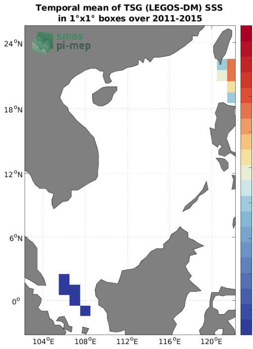
(c) MEAN(TSG (LEGOS-DM) SSS)
