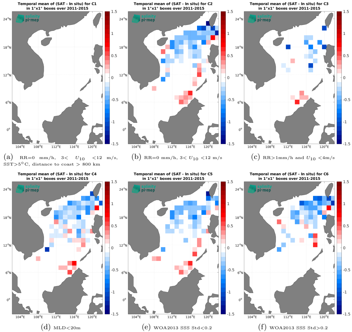
Figure 12: Temporal mean gridded over spatial boxes of size 1^\circ \times 1^\circ of \Delta\text{SSS} (Aquarius SSS L3 OR v5 - 7-Day running - Rain mask (NASA-GSFC) - Argo) for 6 different subdatasets corresponding to: RR=0 mm/h, 3 < U_{10} < 12 m/s, SST > 5^\circ\text{C} , distance to coast > 800 km (a), RR=0 mm/h, 3 < U_{10} < 12 m/s (b), RR > 1 mm/h and U_{10} < 4 m/s (c), MLD < 20 m (d), WOA2013 SSS Std < 0.2 (e), WOA2013 SSS Std > 0.2 (f).
