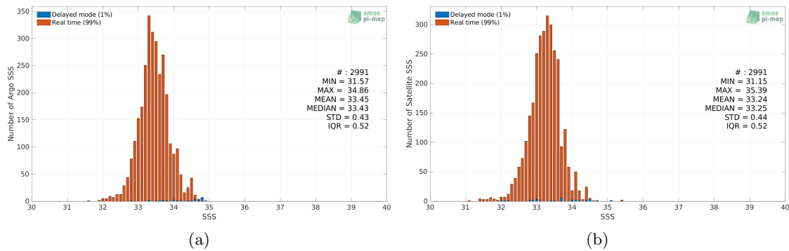
Figure 2: Histograms of SSS from Argo (a) and Aquarius SSS L3 OR v5 - 7-Day running - Rain mask (NASA-GSFC) (b) considering all match-up pairs per bins of 0.1 over the South China Sea Pi-MEP region and for the full satellite product period.
