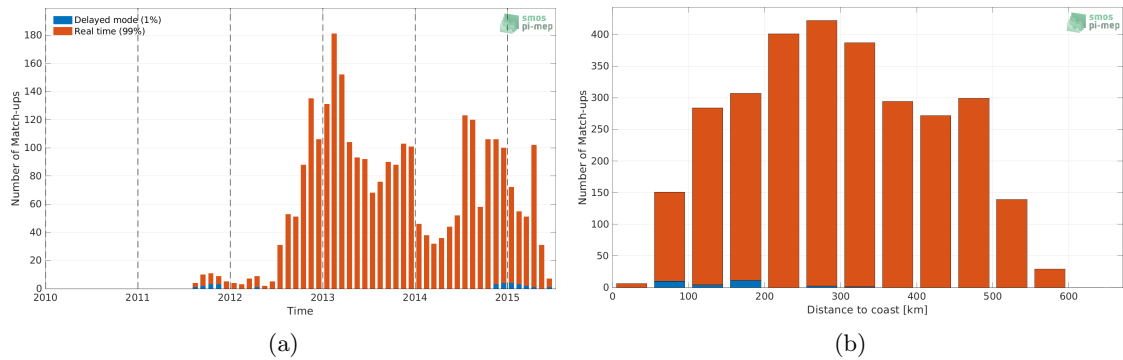
Figure 1: Number of match-ups between Argo and Aquarius SSS L3 OR v5 - 7-Day running - Rain mask (NASA-GSFC) SSS as a function of time (a) and as function of the distance to coast (b) over the South China Sea Pi-MEP region and for the full satellite product period.
