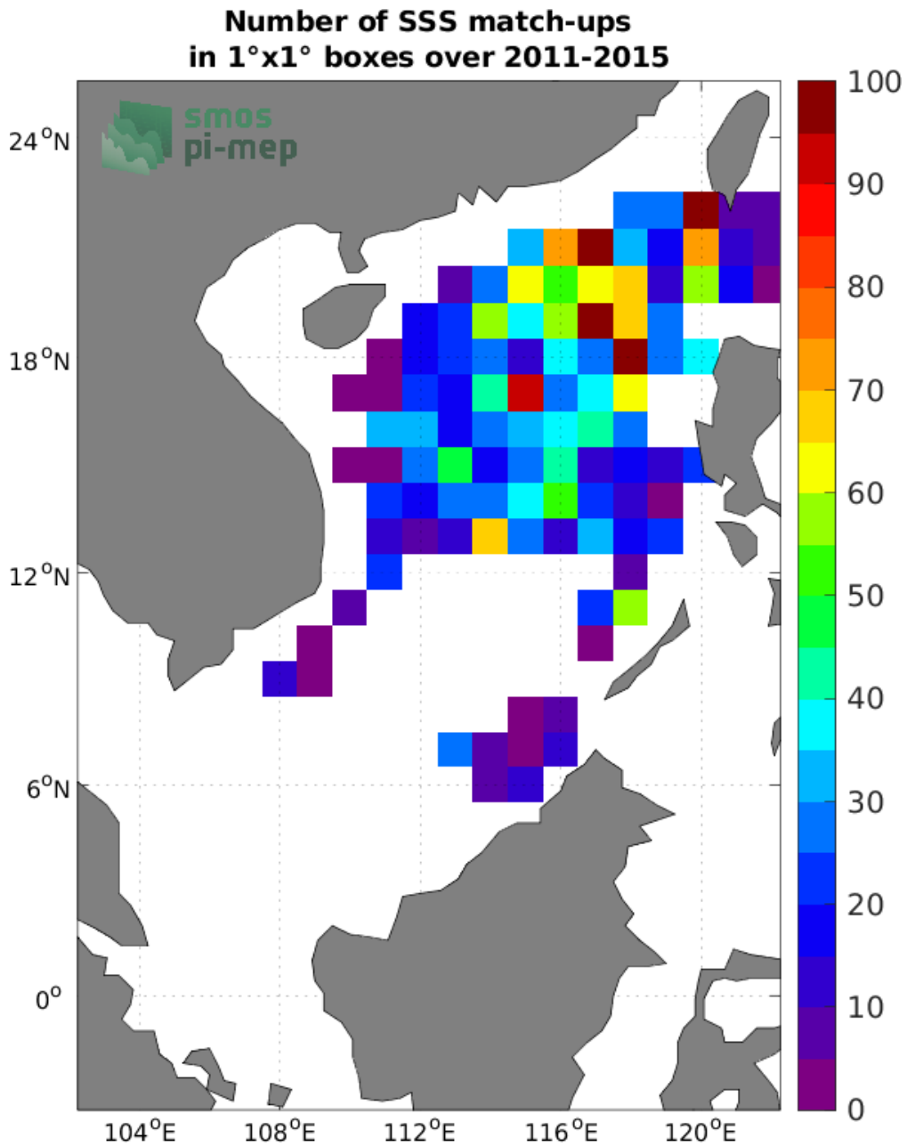
Figure 4: Number of SSS match-ups between Argo SSS and the Aquarius SSS L3 OR v5 - 7-Day running - Rain mask (NASA-GSFC) SSS product for the South China Sea Pi-MEP region over 1°x1° boxes and for the full satellite product period.
