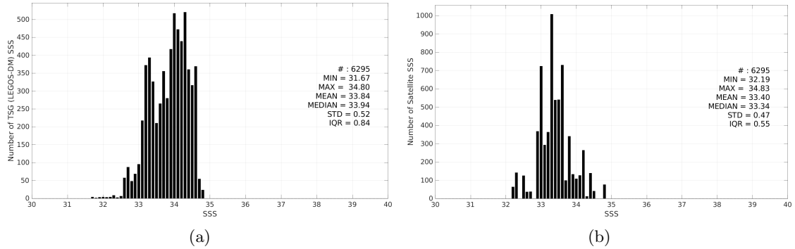
Figure 3: Histograms of SSS from TSG (LEGOS-DM) (a) and Aquarius SSS L3 OR v5 - Monthly (NASA-GSFC) (b) considering all match-up pairs per bins of 0.1 over the South China Sea Pi-MEP region and for the full satellite product period.
