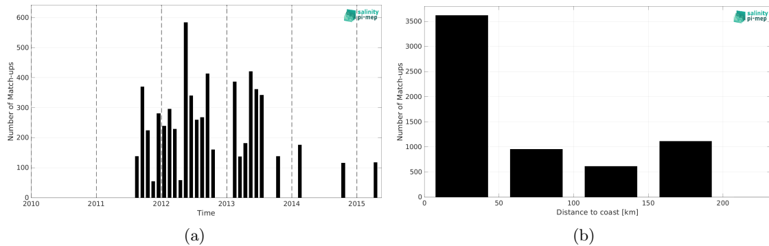
Figure 2: Number of match-ups between TSG (LEGOS-DM) and Aquarius SSS L3 OR v5 - Monthly (NASA-GSFC) SSS as a function of time (a) and as function of the distance to coast (b) over the South China Sea Pi-MEP region and for the full satellite product period.
