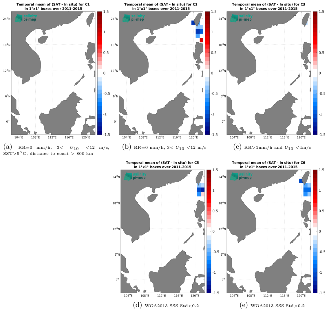
Figure 14: Temporal mean gridded over spatial boxes of size 1^\circ \times 1^\circ of \Delta\text{SSS} (Aquarius SSS L3 OR v5 - Monthly (NASA-GSFC) - TSG (LEGOS-DM)) for 5 different subdatasets corresponding to: RR=0 mm/h, 3 < U_{10} < 12 m/s, SST > 5^\circ\text{C} , distance to coast > 800 km (a), RR=0 mm/h, 3 < U_{10} < 12 m/s (b), RR > 1 mm/h and U_{10} < 4 m/s (c), WOA2013 SSS Std < 0.2 (d), WOA2013 SSS Std > 0.2 (e).
