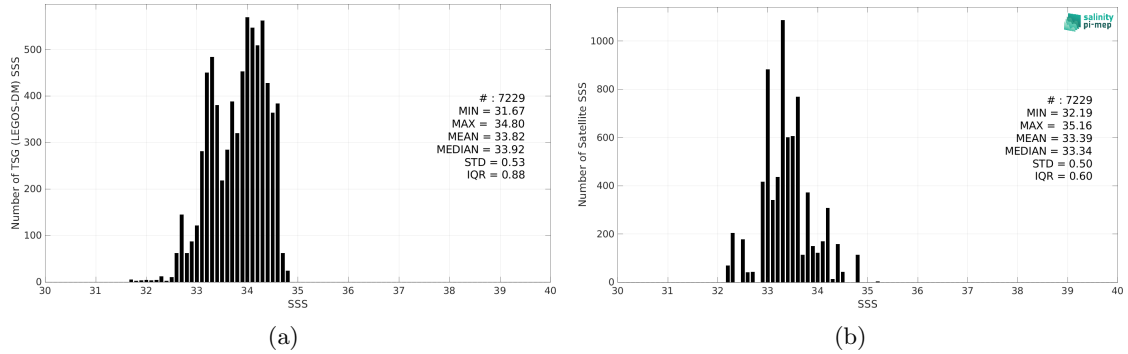
Figure 2: Histograms of SSS from TSG (LEGOS-DM) (a) and Aquarius SSS L3 OR v5 - Monthly (NASA-GSFC) (b) considering all match-up pairs per bins of 0.1 over the South China Sea Pi-MEP region and for the full satellite product period.
