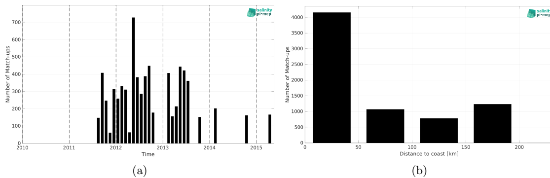
Figure 1: Number of match-ups between TSG (LEGOS-DM) and Aquarius SSS L3 OR v5 - Monthly (NASA-GSFC) SSS as a function of time (a) and as function of the distance to coast (b) over the South China Sea Pi-MEP region and for the full satellite product period.
