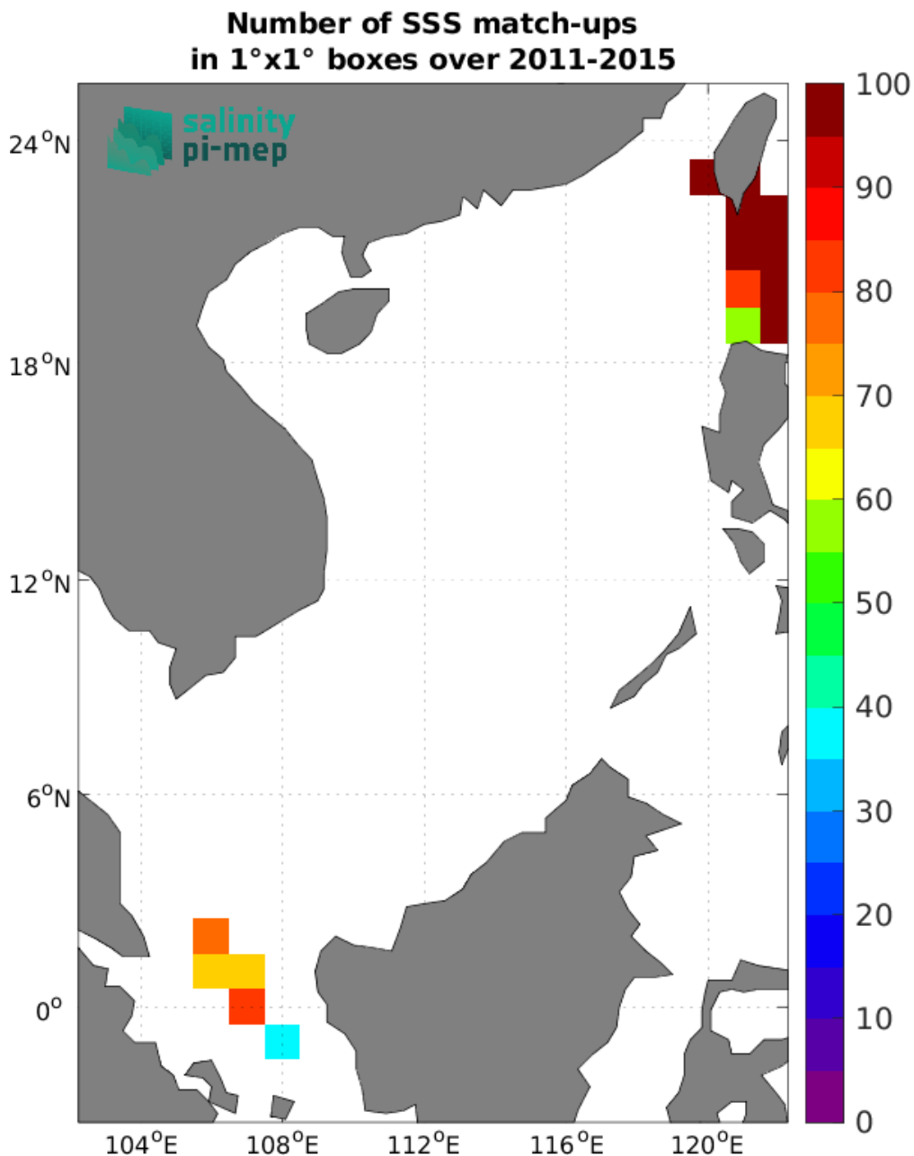
Figure 4: Number of SSS match-ups between TSG (LEGOS-DM) SSS and the Aquarius SSS L3 OR v5 - Monthly (NASA-GSFC) SSS product for the South China Sea Pi-MEP region over 1°x1° boxes and for the full satellite product period.
