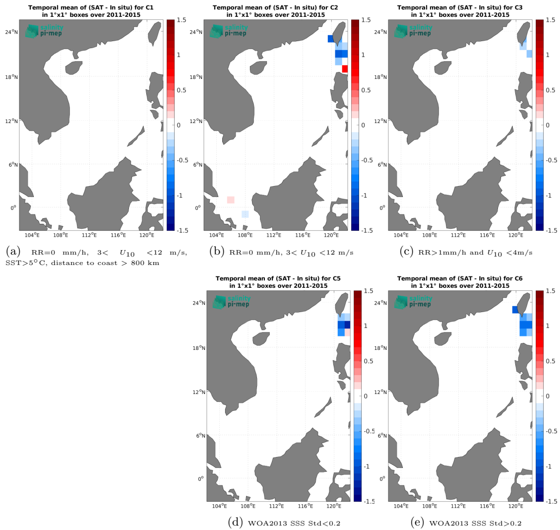
Figure 12: Temporal mean gridded over spatial boxes of size 1^\circ \times 1^\circ of \Delta\text{SSS} (Aquarius SSS L3 OR v5 - Monthly (NASA-GSFC) - TSG (LEGOS-DM)) for 5 different subdatasets corresponding to: RR=0 mm/h, 3 < U_{10} < 12 m/s, SST > 5^\circ\text{C} , distance to coast > 800 km (a), RR=0 mm/h, 3 < U_{10} < 12 m/s (b), RR > 1 mm/h and U_{10} < 4 m/s (c), WOA2013 SSS Std < 0.2 (d), WOA2013 SSS Std > 0.2 (e).
