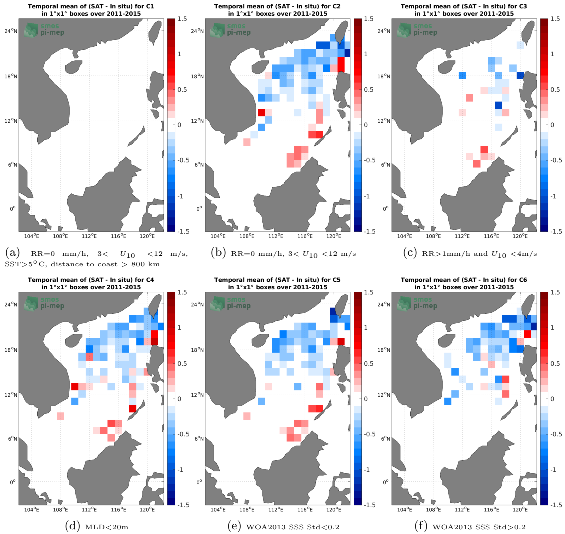
Figure 12: Temporal mean gridded over spatial boxes of size 1^\circ \times 1^\circ of \Delta\text{SSS} (Aquarius SSS L3 OR v5 - Monthly (NASA-GSFC) - Argo) for 6 different subdatasets corresponding to: RR=0 mm/h, 3 < U_{10} < 12 m/s, SST > 5^\circ\text{C} , distance to coast > 800 km (a), RR=0 mm/h, 3 < U_{10} < 12 m/s (b), RR > 1 mm/h and U_{10} < 4 m/s (c), MLD < 20 m (d), WOA2013 SSS Std < 0.2 (e), WOA2013 SSS Std > 0.2 (f).
