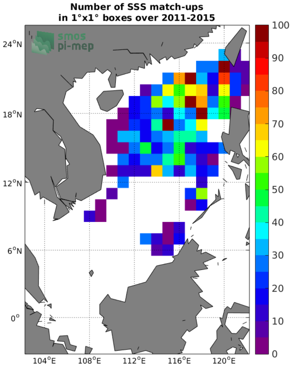
Figure 4: Number of SSS match-ups between Argo SSS and the Aquarius-L3-OR-V5-MONTHLY-1DEG SSS product for the South China Sea Pi-MEP region over 1°x1° boxes and for the full satellite product period.
