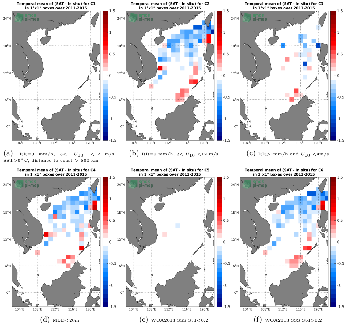
Figure 12: Temporal mean gridded over spatial boxes of size 1°x1° of \Delta SSS (Aquarius-L3-OR-V5-MONTHLY-1DEG - Argo) for 6 different subdatasets corresponding to:RR=0 mm/h, 3 < U_{10} < 12 m/s, SST>5°C, distance to coast > 800 km (a), RR=0 mm/h, 3 < U_{10} < 12 m/s (b), RR>1mm/h and U_{10} < 4 m/s (c),MLD<20m (d),WOA2013 SSS Std<0.2 (e),WOA2013 SSS Std>0.2 (f).
