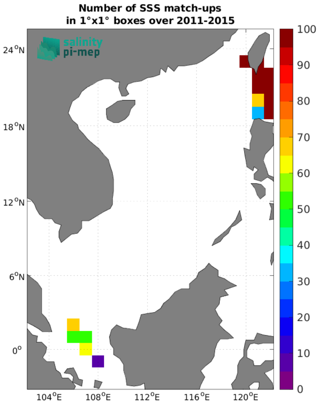
Figure 5: Number of SSS match-ups between TSG (LEGOS-DM) SSS and the Aquarius SSS L3 OR v5 - Monthly - Rain mask (NASA-GSFC) SSS product for the South China Sea Pi-MEP region over 1°x1° boxes and for the full satellite product period.
