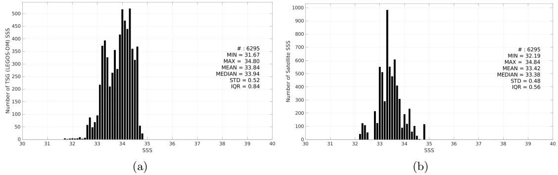
Figure 3: Histograms of SSS from TSG (LEGOS-DM) (a) and Aquarius SSS L3 OR v5 - Monthly - Rain mask (NASA-GSFC) (b) considering all match-up pairs per bins of 0.1 over the South China Sea Pi-MEP region and for the full satellite product period.
