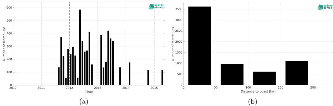
Figure 2: Number of match-ups between TSG (LEGOS-DM) and Aquarius SSS L3 OR v5 - Monthly - Rain mask (NASA-GSFC) SSS as a function of time (a) and as function of the distance to coast (b) over the South China Sea Pi-MEP region and for the full satellite product period.
