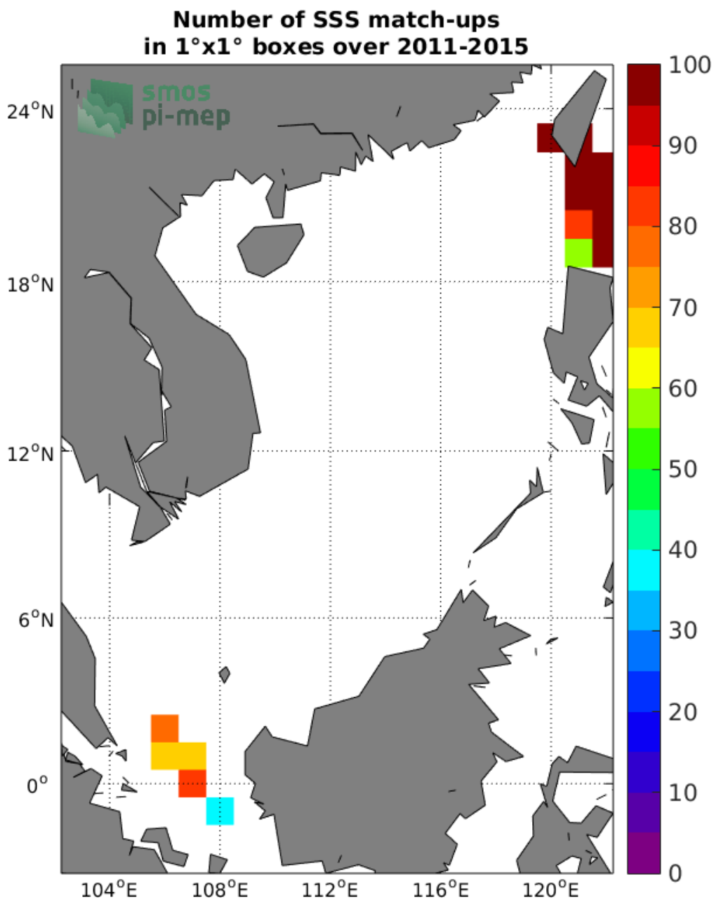
Figure 4: Number of SSS match-ups between TSG-LEGOS-DM SSS and the Aquarius-L3-OR-V5-MONTHLY-RAIN-MASK-1DEG SSS product for the South China Sea Pi-MEP region over 1°x1° boxes and for the full satellite product period.
