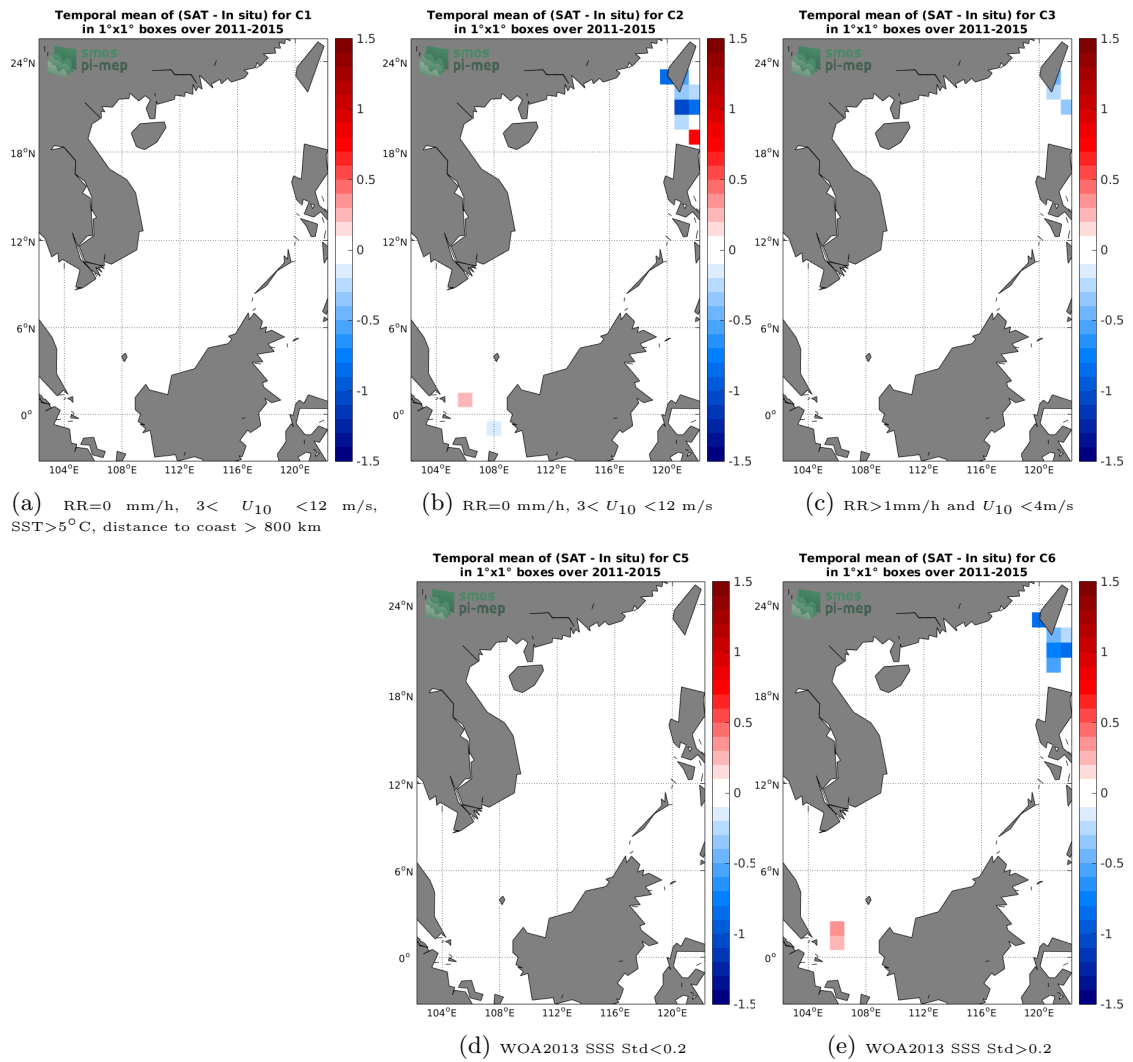
Figure 12: Temporal mean gridded over spatial boxes of size 1^\circ \times 1^\circ of \Delta SSS (Aquarius-L3-OR-V5-MONTHLY-RAIN-MASK-1DEG - TSG-LEGOS-DM) for 5 different subdatasets corresponding to:RR=0 mm/h, 3 < U_{10} < 12 m/s, SST>5°C, distance to coast > 800 km (a), RR=0 mm/h, 3 < U_{10} < 12 m/s (b), RR>1mm/h and U_{10} < 4 m/s (c), WOA2013 SSS Std<0.2 (d), WOA2013 SSS Std>0.2 (e).
