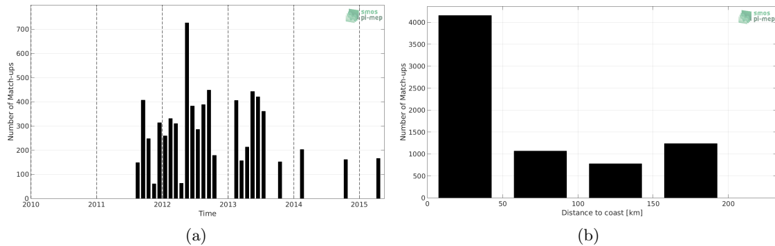
Figure 1: Number of match-ups between TSG-LEGOS-DM and Aquarius-L3-OR-V5-MONTHLY-RAIN-MASK-1DEG SSS as a function of time (a) and as function of the distance to coast (b) over the South China Sea Pi-MEP region and for the full satellite product period.
