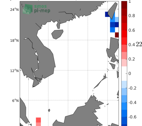
Temporal mean of (Sat-TSG-LEGOS-DM) in 1°x1° boxes over 2011-2015
