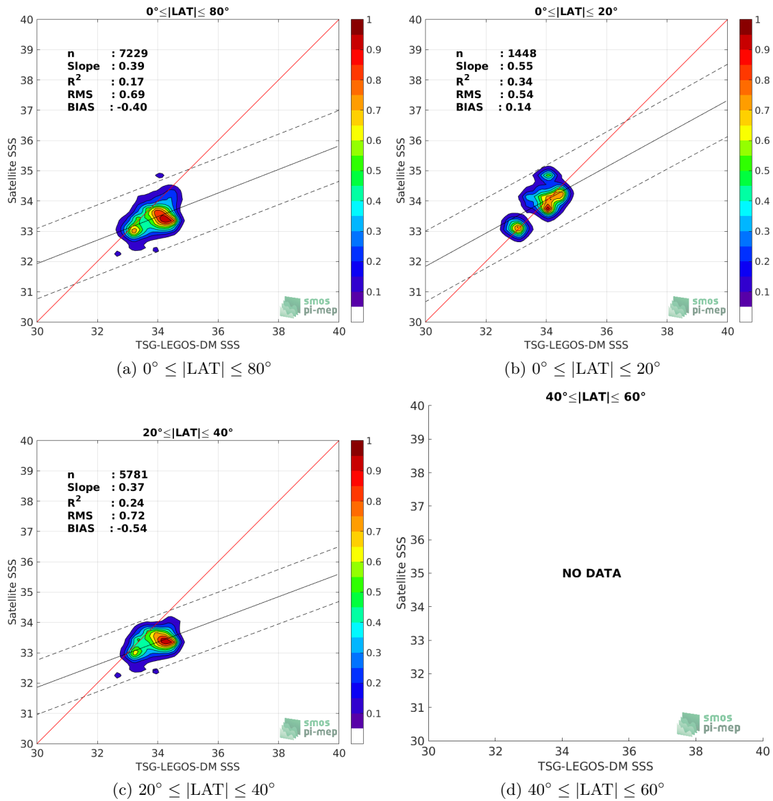
Figure 9: Contour maps of the concentration of Aquarius-L3-OR-V5-MONTHLY-RAIN-MASK-1DEG SSS (y-axis) versus TSG-LEGOS-DM SSS (x-axis) at match-up pairs for different latitude bands. For each plot, the red line shows x=y . The black thin and dashed lines indicate a linear fit through the data cloud and the \pm 95\% confidence levels, respectively. The number match-up pairs n , the slope and R^2 coefficient of the linear fit, the root mean square (RMS) and the mean bias between satellite and in situ data are indicated for each latitude band in each plots.
