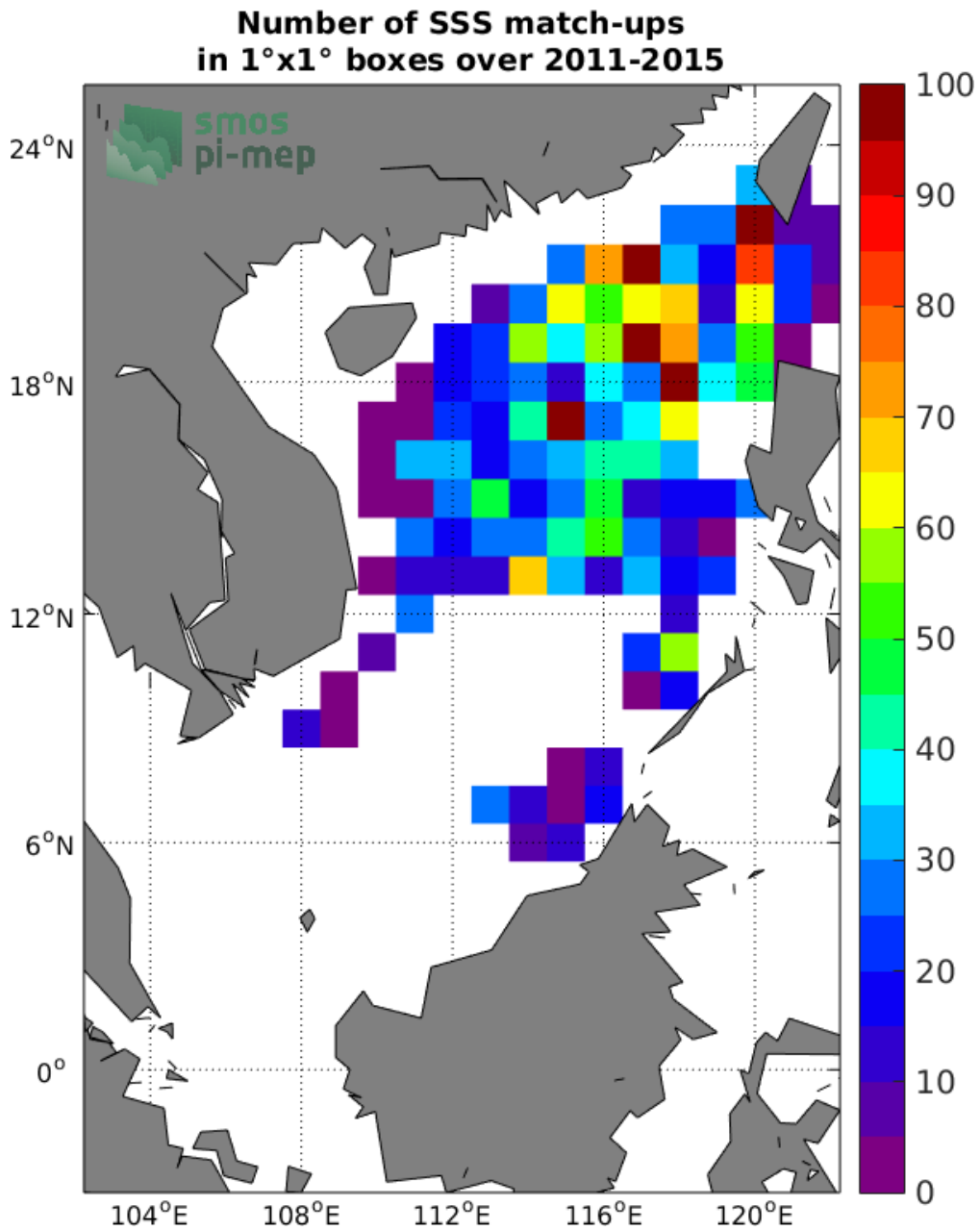
Figure 4: Number of SSS match-ups between Argo SSS and the Aquarius-L3-OR-V5-MONTHLY-RAIN-MASK-1DEG SSS product for the South China Sea Pi-MEP region over 1°x1° boxes and for the full satellite product period.
