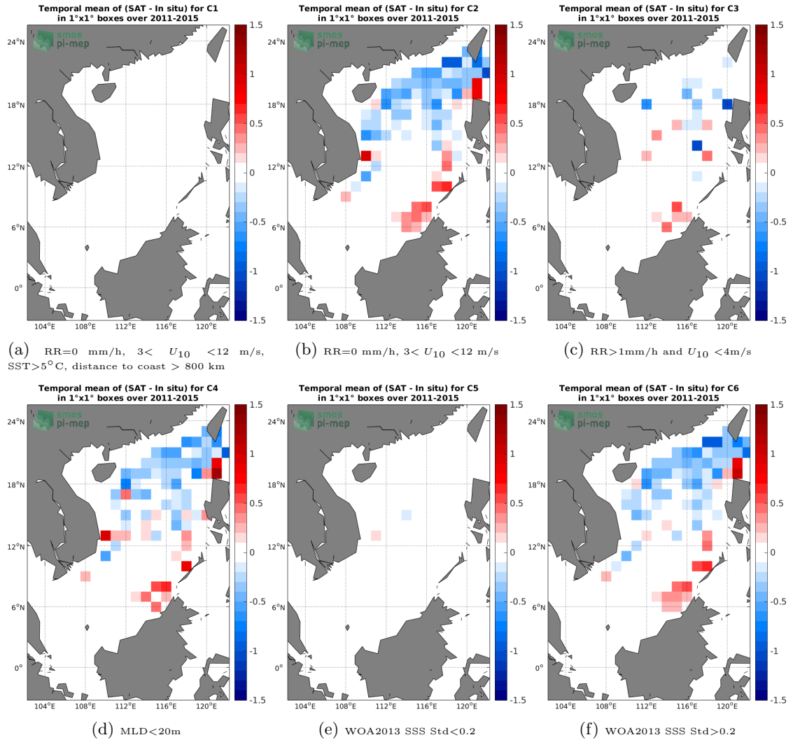
Figure 12: Temporal mean gridded over spatial boxes of size 1°x1° of \Delta SSS (Aquarius-L3-OR-V5-MONTHLY-RAIN-MASK-1DEG - Argo) for 6 different subdatasets corresponding to:RR=0 mm/h, 3 < U_{10} < 12 m/s, SST>5°C, distance to coast > 800 km (a), RR=0 mm/h, 3 < U_{10} < 12 m/s (b), RR>1mm/h and U_{10} < 4 m/s (c),MLD<20m (d),WOA2013 SSS Std<0.2 (e),WOA2013 SSS Std>0.2 (f).
