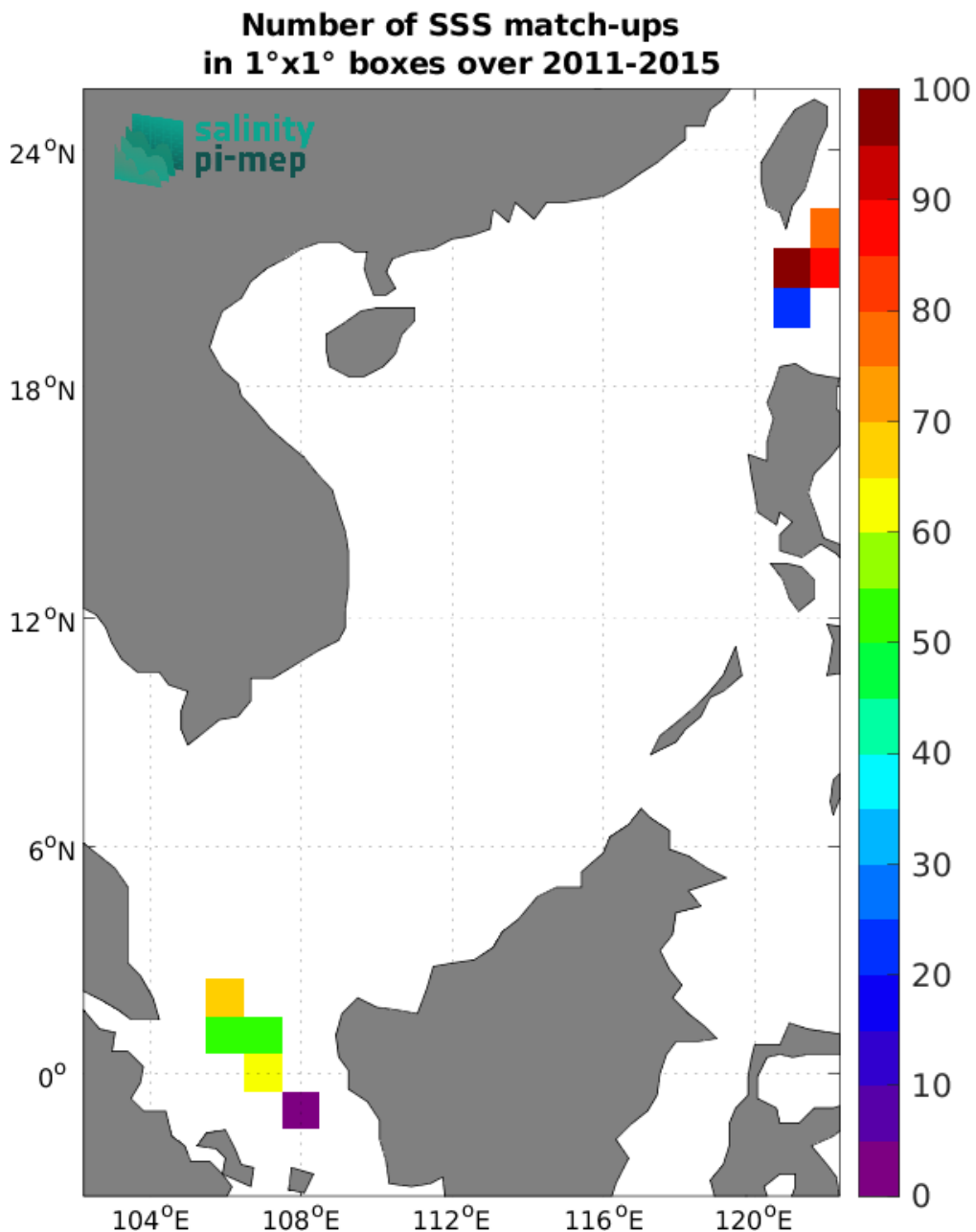
Figure 5: Number of SSS match-ups between TSG (LEGOS-DM) SSS and the Aquarius SSS L3 CAP v5 - 7-Day running (JPL) SSS product for the South China Sea Pi-MEP region over 1°x1° boxes and for the full satellite product period.
