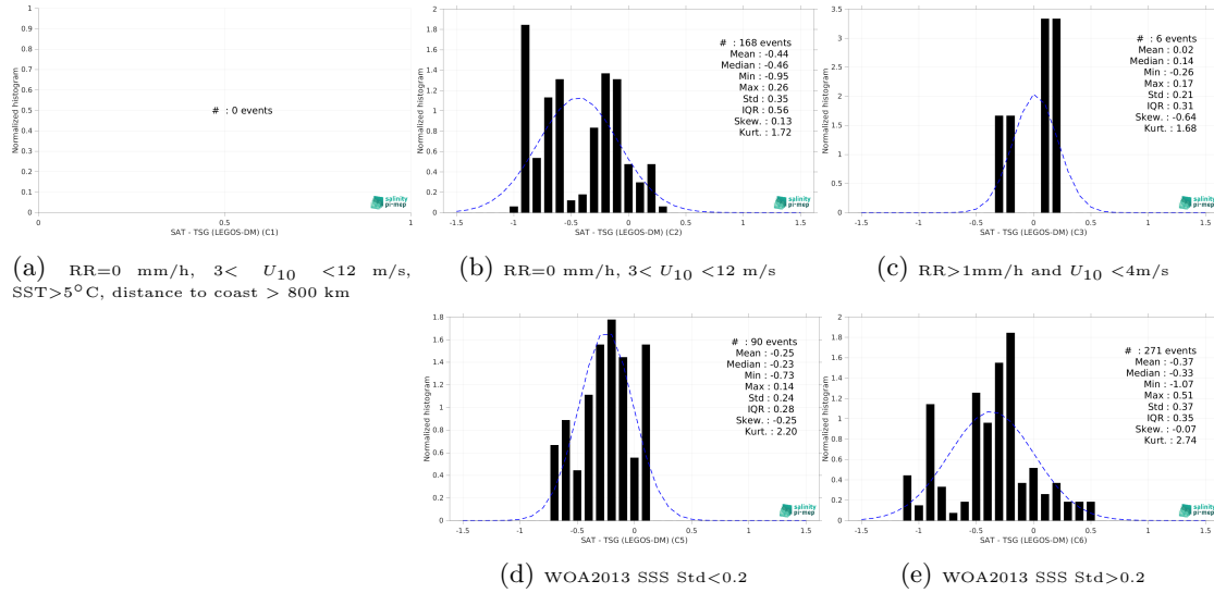
Figure 15: Normalized histogram of \Delta SSS (Aquarius SSS L3 CAP v5 - 7-Day running (JPL) - TSG (LEGOS-DM)) for 5 different subdatasets corresponding to: RR=0 mm/h, 3 < U_{10} < 12 m/s, SST > 5°C, distance to coast > 800 km (a), RR=0 mm/h, 3 < U_{10} < 12 m/s (b), RR > 1mm/h and U_{10} < 4 m/s (c), WOA2013 SSS Std < 0.2 (d), WOA2013 SSS Std > 0.2 (e).
