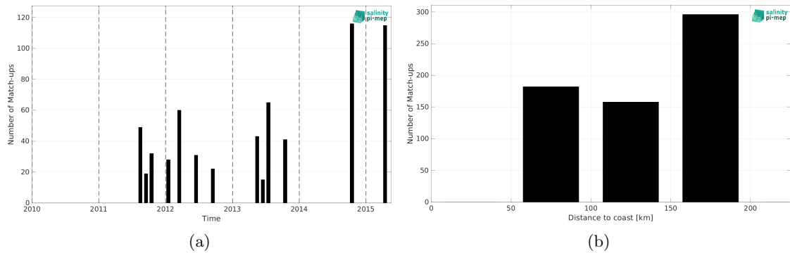
Figure 2: Number of match-ups between TSG (LEGOS-DM) and Aquarius SSS L3 CAP v5 - 7-Day running (JPL) SSS as a function of time (a) and as function of the distance to coast (b) over the South China Sea Pi-MEP region and for the full satellite product period.
