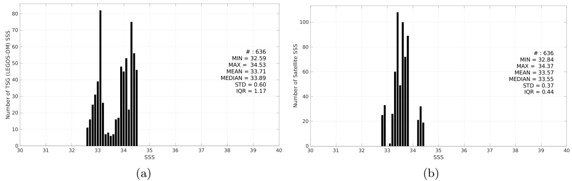
Figure 3: Histograms of SSS from TSG (LEGOS-DM) (a) and Aquarius SSS L3 CAP v5 - 7-Day running (JPL) (b) considering all match-up pairs per bins of 0.1 over the South China Sea Pi-MEP region and for the full satellite product period.
