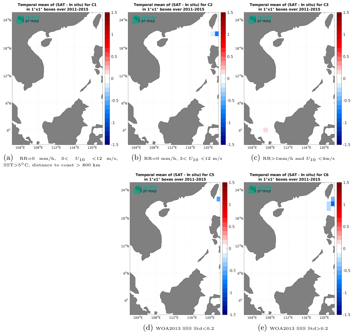
Figure 14: Temporal mean gridded over spatial boxes of size 1^\circ \times 1^\circ of \Delta\text{SSS} (Aquarius SSS L3 CAP v5 - 7-Day running (JPL) - TSG (LEGOS-DM)) for 5 different subdatasets corresponding to: RR=0 mm/h, 3 < U_{10} < 12 m/s, SST > 5^\circ\text{C} , distance to coast > 800 km (a), RR=0 mm/h, 3 < U_{10} < 12 m/s (b), RR > 1 mm/h and U_{10} < 4 m/s (c), WOA2013 SSS Std < 0.2 (d), WOA2013 SSS Std > 0.2 (e).
