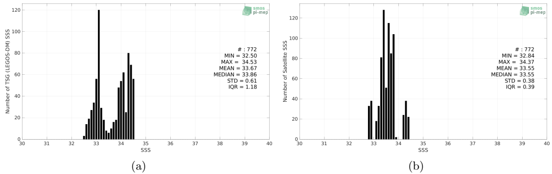
Figure 2: Histograms of SSS from TSG (LEGOS-DM) (a) and Aquarius SSS L3 CAP v5 - 7-Day running (JPL) (b) considering all match-up pairs per bins of 0.1 over the South China Sea Pi-MEP region and for the full satellite product period.
