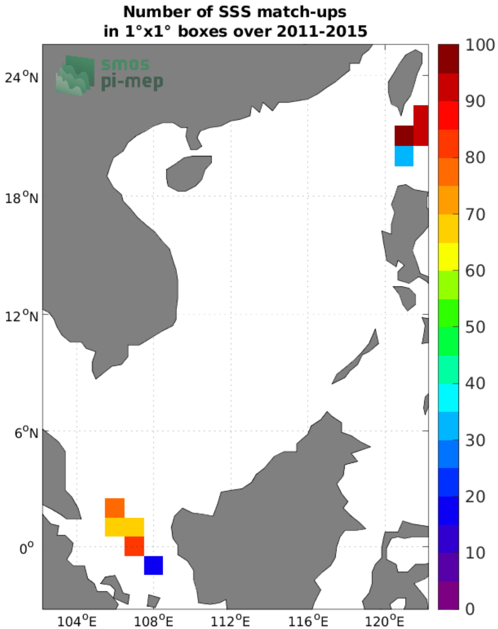
Figure 4: Number of SSS match-ups between TSG (LEGOS-DM) SSS and the Aquarius SSS L3 CAP v5 - 7-Day running (JPL) SSS product for the South China Sea Pi-MEP region over 1^\circ \times 1^\circ boxes and for the full satellite product period.
