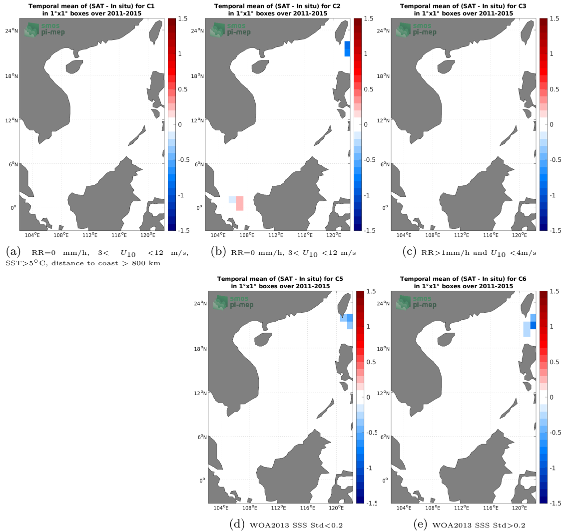
Figure 12: Temporal mean gridded over spatial boxes of size 1^\circ \times 1^\circ of \Delta SSS (Aquarius SSS L3 CAP v5 - 7-Day running (JPL) - TSG (LEGOS-DM)) for 5 different subdatasets corresponding to:RR=0 mm/h, 3 < U_{10} < 12 m/s, SST>5°C, distance to coast > 800 km (a), RR=0 mm/h, 3 < U_{10} < 12 m/s (b), RR>1mm/h and U_{10} < 4 m/s (c), WOA2013 SSS Std<0.2 (d), WOA2013 SSS Std>0.2 (e).
