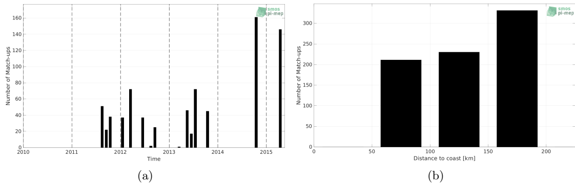
Figure 1: Number of match-ups between TSG (LEGOS-DM) and Aquarius SSS L3 CAP v5 - 7-Day running (JPL) SSS as a function of time (a) and as function of the distance to coast (b) over the South China Sea Pi-MEP region and for the full satellite product period.
