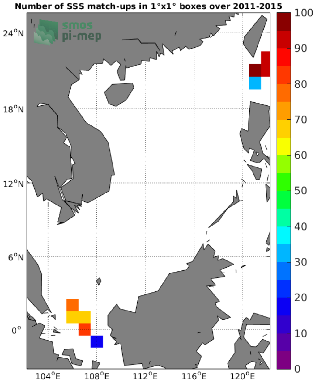
Figure 4: Number of SSS match-ups between TSG-LEGOS-DM SSS and the Aquarius-L3-JPL-V5-7DAY-RUNNING SSS product for the South China Sea Pi-MEP region over 1°x1° boxes and for the full satellite product period.
