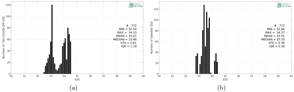
Figure 2: Histograms of SSS from TSG-LEGOS-DM (a) and Aquarius-L3-JPL-V5-7DAY-RUNNING (b) considering all match-up pairs per bins of 0.1 over the South China Sea Pi-MEP region and for the full satellite product period.
