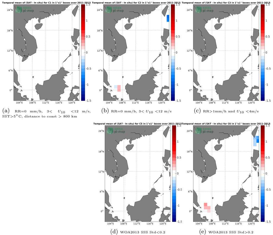
Figure 12: Temporal mean gridded over spatial boxes of size 1^\circ \times 1^\circ of \Delta SSS (Aquarius-L3-JPL-V5-7DAY-RUNNING - TSG-LEGOS-DM) for 5 different subdatasets corresponding to: RR=0 mm/h, 3 < U_{10} < 12 m/s, SST > 5^\circ C , distance to coast > 800 km (a), RR=0 mm/h, 3 < U_{10} < 12 m/s (b), RR > 1 mm/h and U_{10} < 4 m/s (c), WOA2013 SSS Std < 0.2 (d), WOA2013 SSS Std > 0.2 (e).
