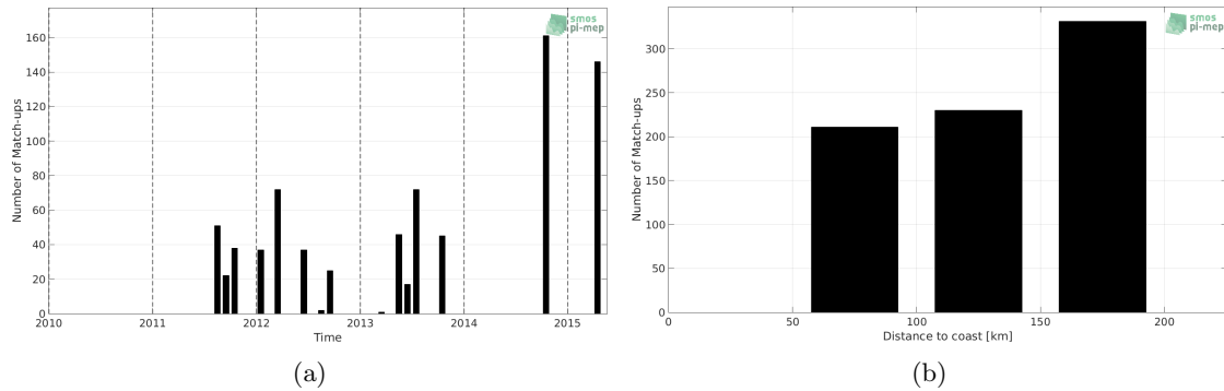
Figure 1: Number of match-ups between TSG-LEGOS-DM and Aquarius-L3-JPL-V5-7DAY-RUNNING SSS as a function of time (a) and as function of the distance to coast (b) over the South China Sea Pi-MEP region and for the full satellite product period.
