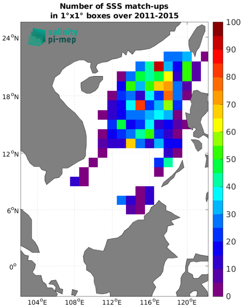
Figure 4: Number of SSS match-ups between Argo SSS and the Aquarius SSS L3 CAP v5 - 7-Day running (JPL) SSS product for the South China Sea Pi-MEP region over 1^\circ \times 1^\circ boxes and for the full satellite product period.
