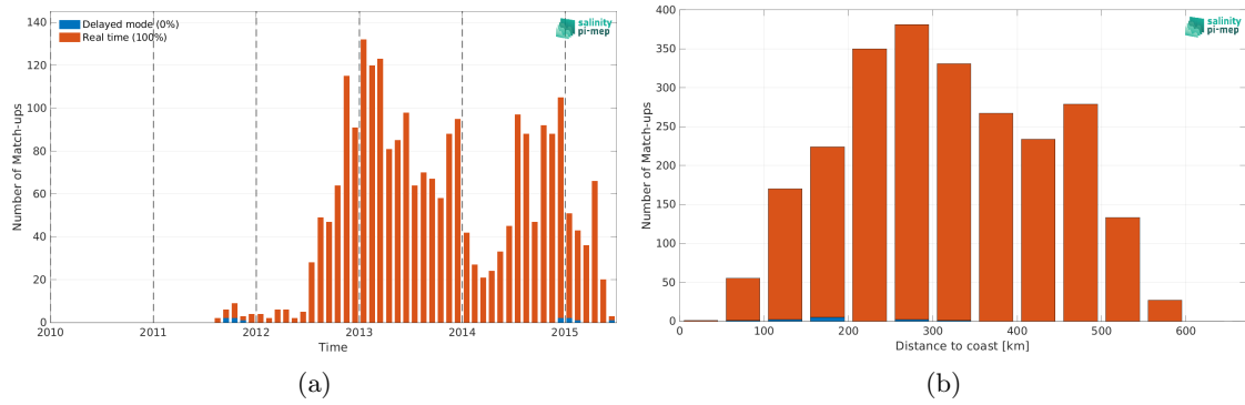
Figure 1: Number of match-ups between Argo and Aquarius SSS L3 CAP v5 - 7-Day running (JPL) SSS as a function of time (a) and as function of the distance to coast (b) over the South China Sea Pi-MEP region and for the full satellite product period.
