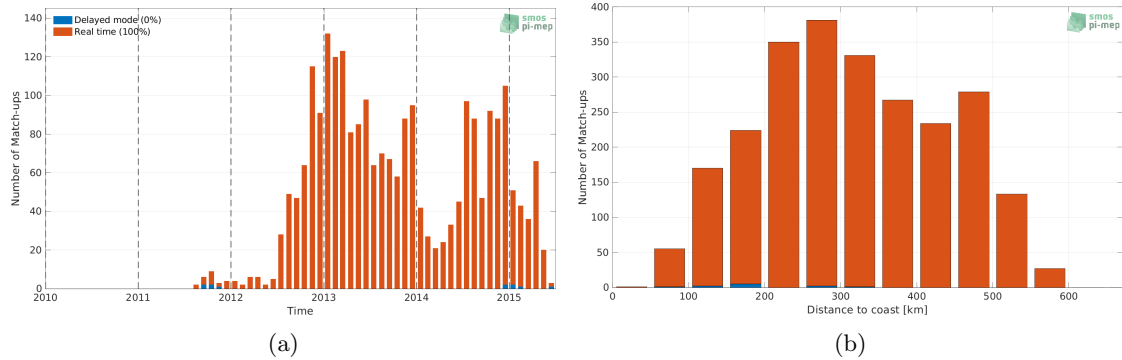
Figure 1: Number of match-ups between Argo and Aquarius SSS L3 CAP v5 - 7-Day running (JPL) SSS as a function of time (a) and as function of the distance to coast (b) over the South China Sea Pi-MEP region and for the full satellite product period.
