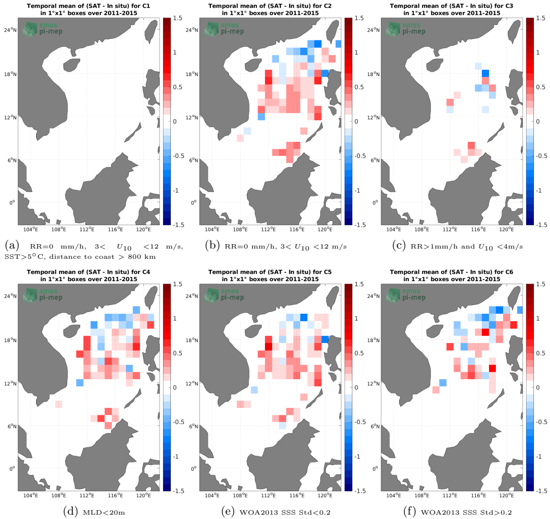
Figure 12: Temporal mean gridded over spatial boxes of size 1^\circ \times 1^\circ of \Delta SSS (Aquarius SSS L3 CAP v5 - 7-Day running (JPL) - Argo) for 6 different subdatasets corresponding to:RR=0 mm/h, 3 < U_{10} < 12 m/s, SST>5°C, distance to coast > 800 km (a), RR=0 mm/h, 3 < U_{10} < 12 m/s (b), RR>1mm/h and U_{10} < 4 m/s (c),MLD<20m (d),WOA2013 SSS Std<0.2 (e),WOA2013 SSS Std>0.2 (f).
