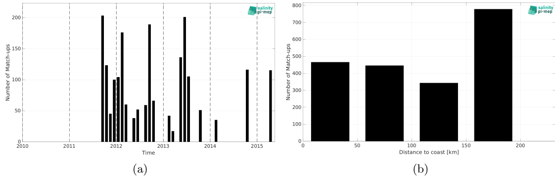
Figure 2: Number of match-ups between TSG (LEGOS-DM) and Aquarius SSS L3 CAP v5 - Monthly (JPL) SSS as a function of time (a) and as function of the distance to coast (b) over the South China Sea Pi-MEP region and for the full satellite product period.
