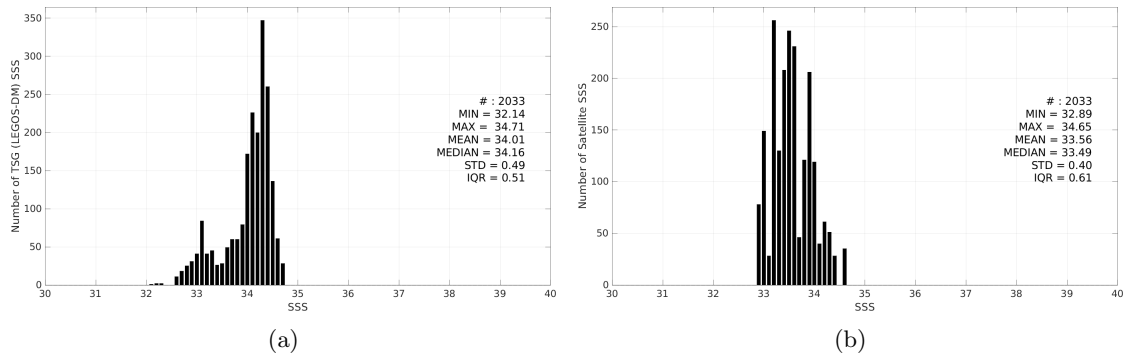
Figure 3: Histograms of SSS from TSG (LEGOS-DM) (a) and Aquarius SSS L3 CAP v5 - Monthly (JPL) (b) considering all match-up pairs per bins of 0.1 over the South China Sea Pi-MEP region and for the full satellite product period.
