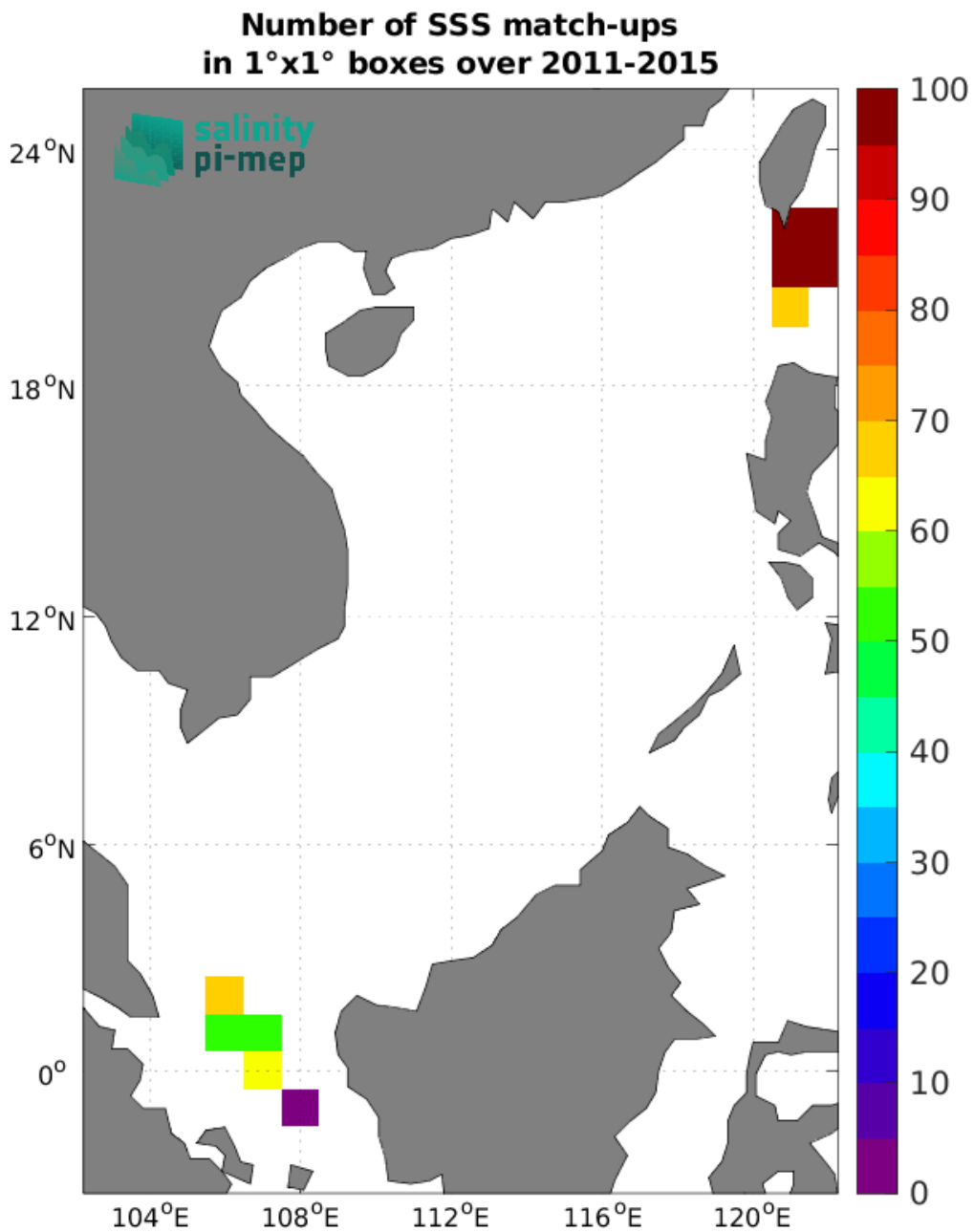
Figure 5: Number of SSS match-ups between TSG (LEGOS-DM) SSS and the Aquarius SSS L3 CAP v5 - Monthly (JPL) SSS product for the South China Sea Pi-MEP region over 1^\circ \times 1^\circ boxes and for the full satellite product period.
