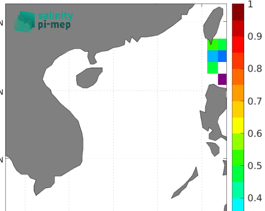
Temporal STD of (Sat - TSG (LEGOS-DM)) in 1°x1° boxes over 2011-2015
