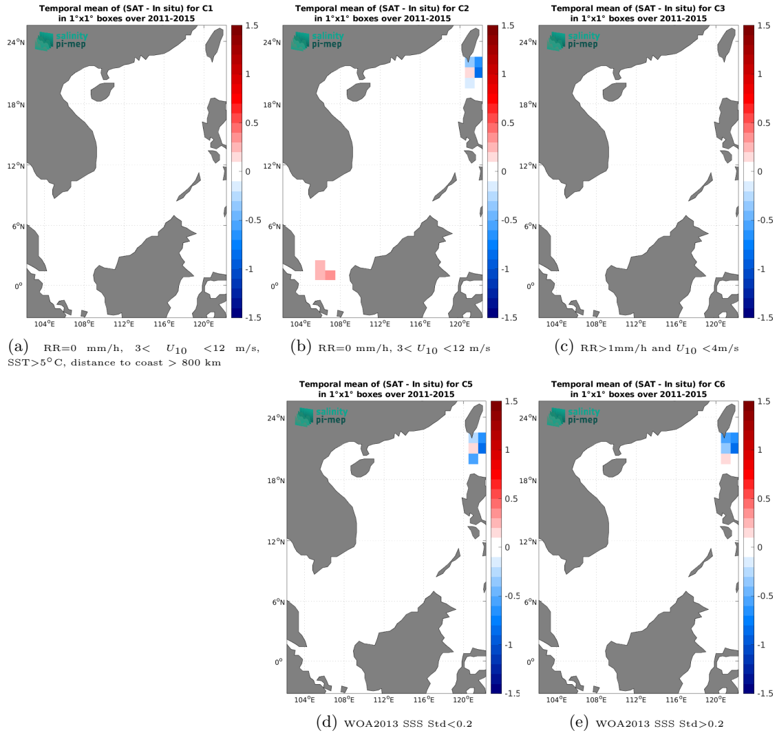
Figure 12: Temporal mean gridded over spatial boxes of size 1^\circ \times 1^\circ of \Delta\text{SSS} (Aquarius SSS L3 CAP v5 - Monthly (JPL) - TSG (LEGOS-DM)) for 5 different subdatasets corresponding to: RR=0 mm/h, 3 < U_{10} < 12 m/s, SST > 5^\circ\text{C} , distance to coast > 800 km (a), RR=0 mm/h, 3 < U_{10} < 12 m/s (b), RR > 1 mm/h and U_{10} < 4 m/s (c), WOA2013 SSS Std < 0.2 (d), WOA2013 SSS Std > 0.2 (e).
