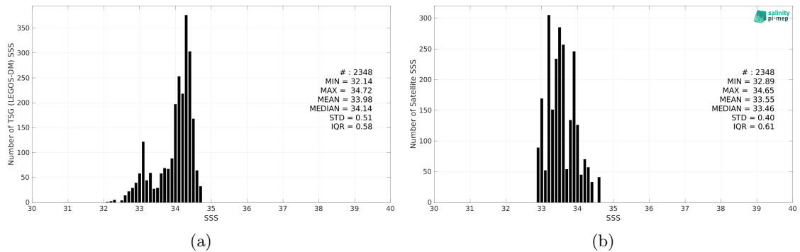
Figure 2: Histograms of SSS from TSG (LEGOS-DM) (a) and Aquarius SSS L3 CAP v5 - Monthly (JPL) (b) considering all match-up pairs per bins of 0.1 over the South China Sea Pi-MEP region and for the full satellite product period.
