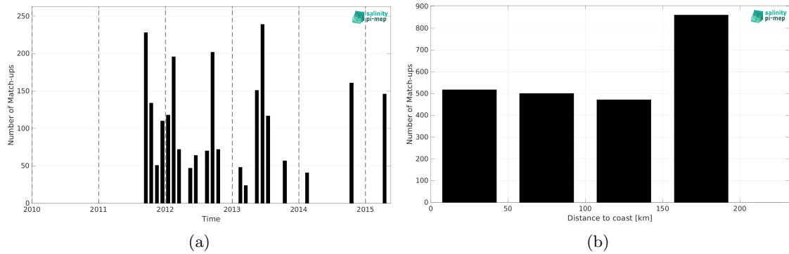
Figure 1: Number of match-ups between TSG (LEGOS-DM) and Aquarius SSS L3 CAP v5 - Monthly (JPL) SSS as a function of time (a) and as function of the distance to coast (b) over the South China Sea Pi-MEP region and for the full satellite product period.
