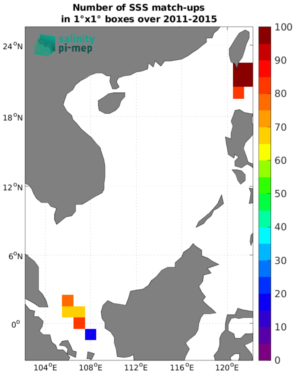
Figure 4: Number of SSS match-ups between TSG (LEGOS-DM) SSS and the Aquarius SSS L3 CAP v5 - Monthly (JPL) SSS product for the South China Sea Pi-MEP region over 1^\circ \times 1^\circ boxes and for the full satellite product period.
