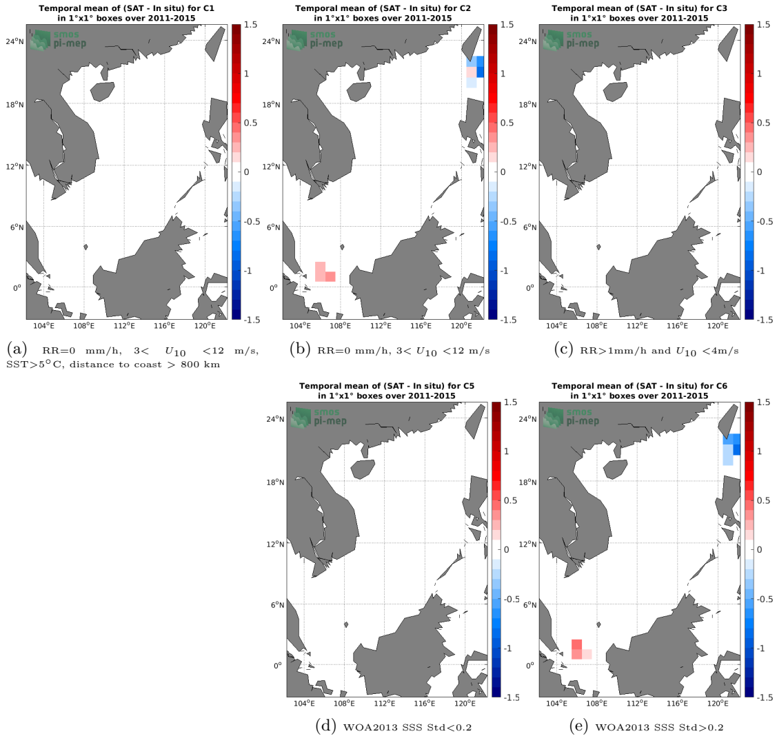
Figure 12: Temporal mean gridded over spatial boxes of size 1^\circ \times 1^\circ of \Delta SSS (Aquarius SSS L3 CAP v5 - Monthly (JPL) - TSG (LEGOS-DM)) for 5 different subdatasets corresponding to:RR=0 mm/h, 3 < U_{10} < 12 m/s, SST>5°C, distance to coast > 800 km (a), RR=0 mm/h, 3 < U_{10} < 12 m/s (b), RR>1mm/h and U_{10} < 4 m/s (c), WOA2013 SSS Std<0.2 (d), WOA2013 SSS Std>0.2 (e).
