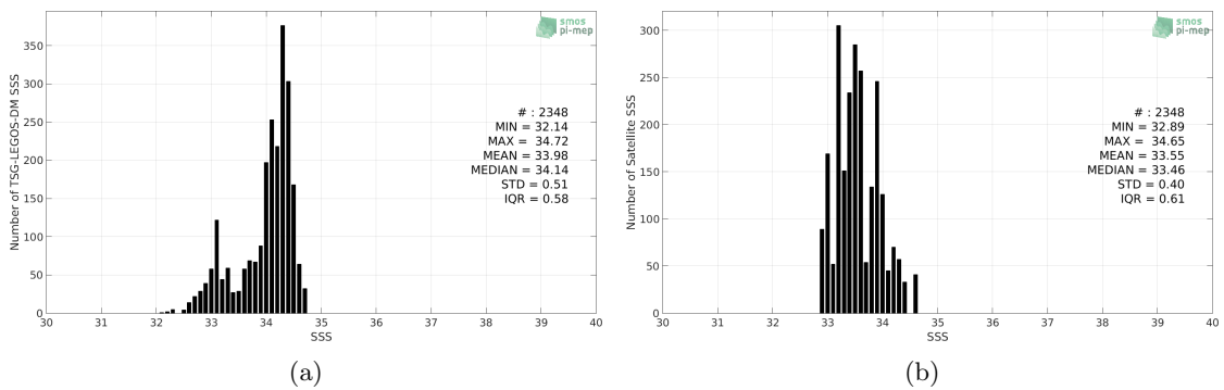
Figure 2: Histograms of SSS from TSG-LEGOS-DM (a) and Aquarius-L3-JPL-V5-MONTHLY (b) considering all match-up pairs per bins of 0.1 over the South China Sea Pi-MEP region and for the full satellite product period.
