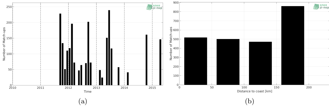
Figure 1: Number of match-ups between TSG-LEGOS-DM and Aquarius-L3-JPL-V5-MONTHLY SSS as a function of time (a) and as function of the distance to coast (b) over the South China Sea Pi-MEP region and for the full satellite product period.
