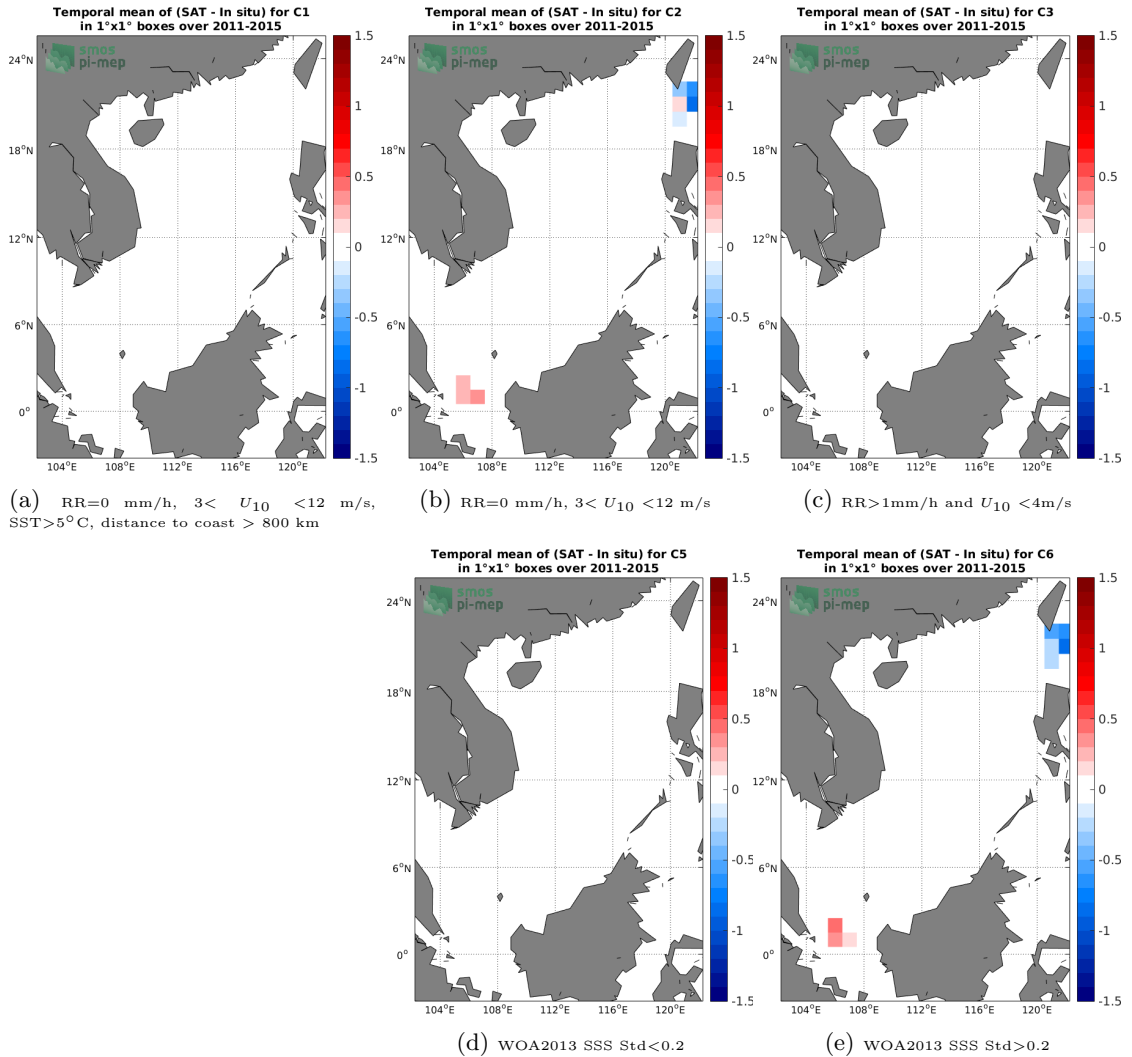
Figure 12: Temporal mean gridded over spatial boxes of size 1^\circ \times 1^\circ of \Delta SSS (Aquarius-L3-JPL-V5-MONTHLY - TSG-LEGOS-DM) for 5 different subdatasets corresponding to:RR=0 mm/h, 3 < U_{10} < 12 m/s, SST >5^\circ\text{C} , distance to coast > 800 km (a), RR=0 mm/h, 3 < U_{10} < 12 m/s (b), RR >1 mm/h and U_{10} < 4 m/s (c), WOA2013 SSS Std <0.2 (d), WOA2013 SSS Std >0.2 (e).
