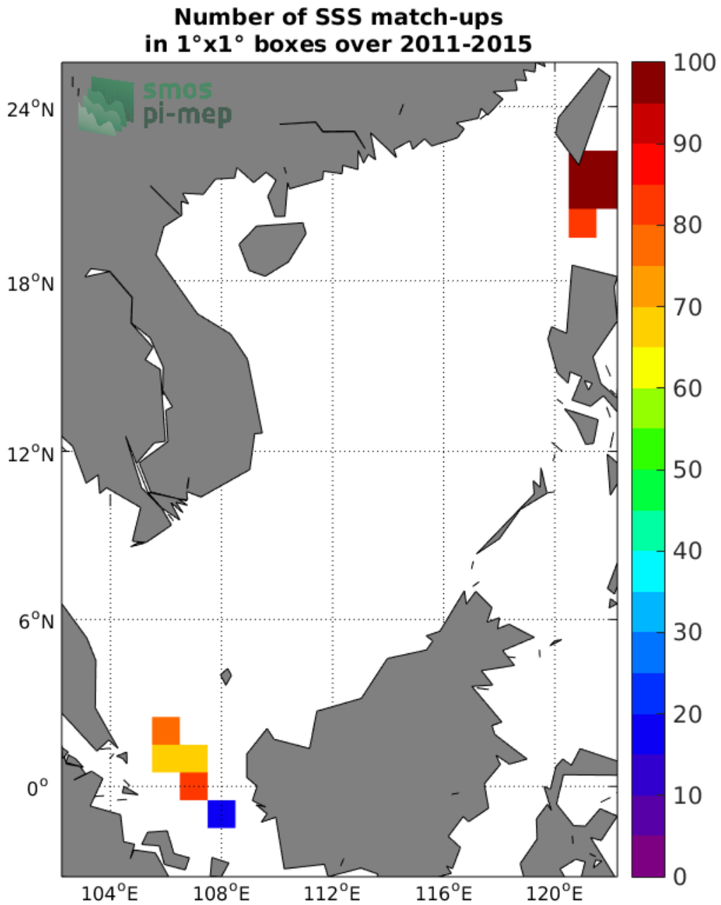
Figure 4: Number of SSS match-ups between TSG-LEGOS-DM SSS and the Aquarius-L3-JPL-V5-MONTHLY SSS product for the South China Sea Pi-MEP region over 1°x1° boxes and for the full satellite product period.
