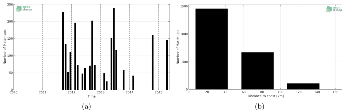
Figure 1: Number of match-ups between TSG-LEGOS-DM and Aquarius-L3-JPL-V5-MONTHLY SSS as a function of time (a) and as function of the distance to coast (b) over the South China Sea Pi-MEP region and for the full satellite product period.
