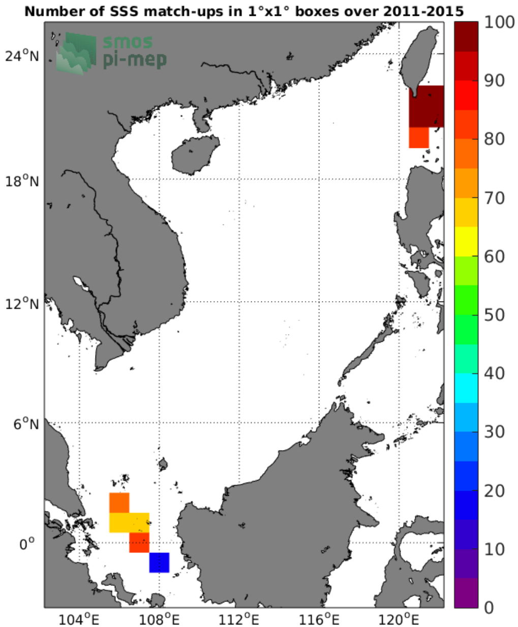
Figure 4: Number of SSS match-ups between TSG-LEGOS-DM SSS and the Aquarius-L3-JPL-V5-MONTHLY SSS product for the South China Sea Pi-MEP region over 1°x1° boxes and for the full satellite product period.
