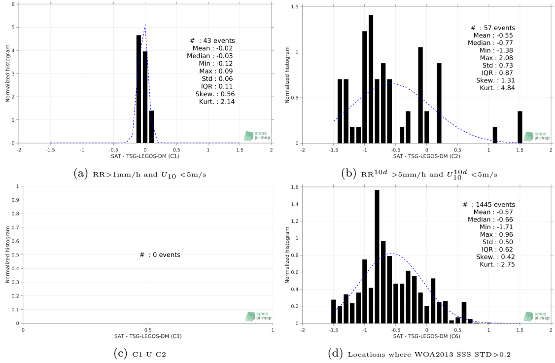
Figure 13: Normalized histogram of \Delta\text{SSS} (Aquarius-L3-JPL-V5-MONTHLY - TSG-LEGOS-DM) for 6 different subdatasets corresponding to: RR > 1mm/h and U_{10} < 5\text{m/s} (a), RR^{10d} > 5\text{mm/h} and U_{10}^{10d} < 5\text{m/s} (b), C1 U C2 (c), Locations where WOA2013 SSS STD > 0.2 (d).
