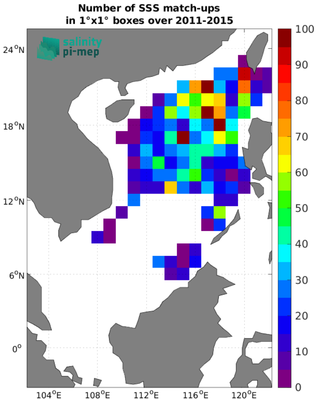
Figure 4: Number of SSS match-ups between Argo SSS and the Aquarius SSS L3 CAP v5 - Monthly (JPL) SSS product for the South China Sea Pi-MEP region over 1^\circ \times 1^\circ boxes and for the full satellite product period.
