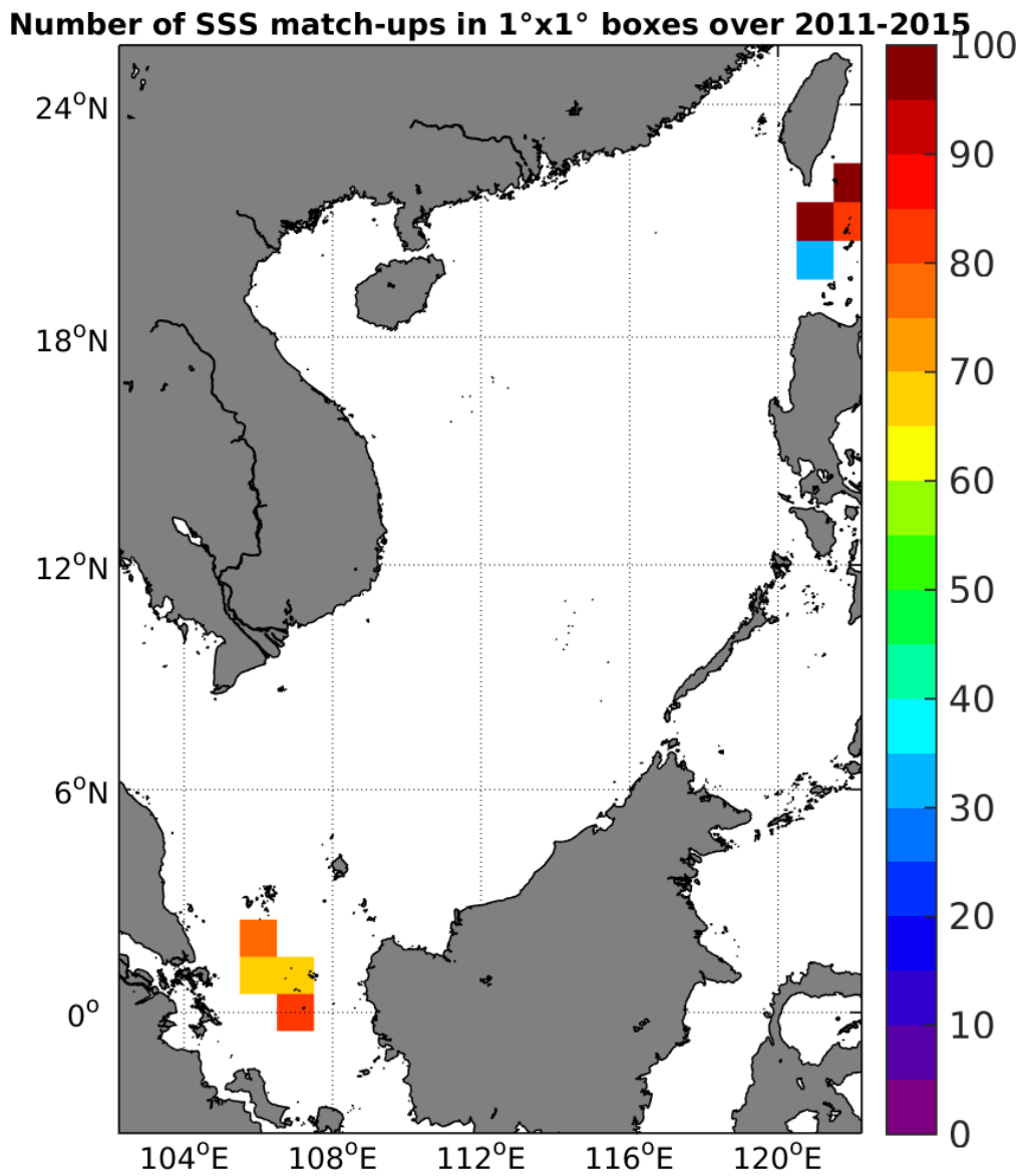
Figure 4: Number of SSS match-ups between TSG-LEGOS-DM SSS and the Aquarius-L3-JPL-V4-7DAY-RUNNING SSS product for the South China Sea Pi-MEP region over 1°x1° boxes and for the full satellite product period.
