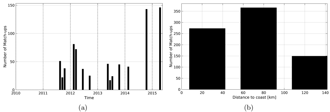
Figure 1: Number of match-ups between TSG-LEGOS-DM and Aquarius-L3-JPL-V4-7DAY-RUNNING SSS as a function of time (a) and as function of the distance to coast (b) over the South China Sea Pi-MEP region and for the full satellite product period.
