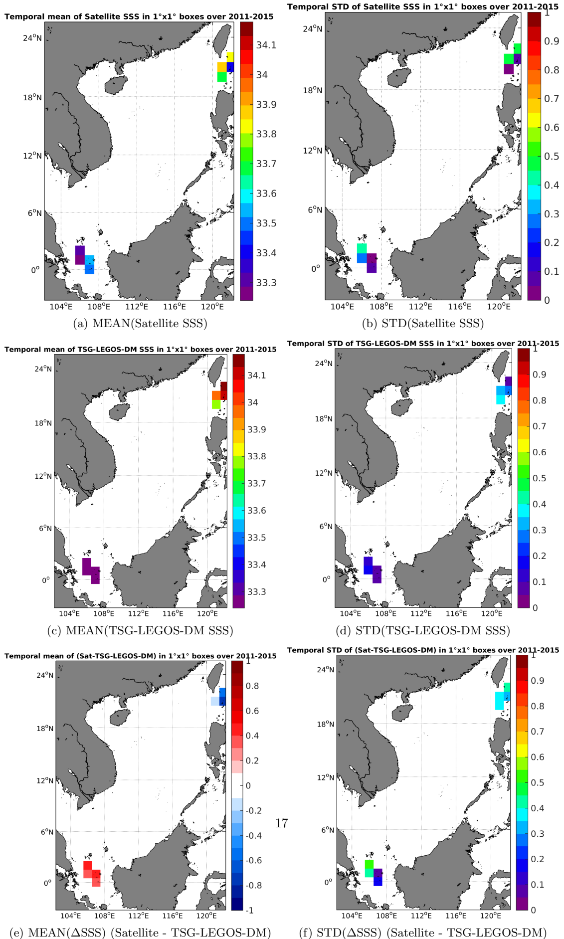
Figure 6: Temporal mean (left) and STD (right) of SSS from Aquarius-L3-JPL-V4-7DAY-RUNNING (top), TSG-LEGOS-DM (middle), and of \Delta SSS (Satellite - TSG-LEGOS-DM). Only match-up pairs are used to generate these maps.
