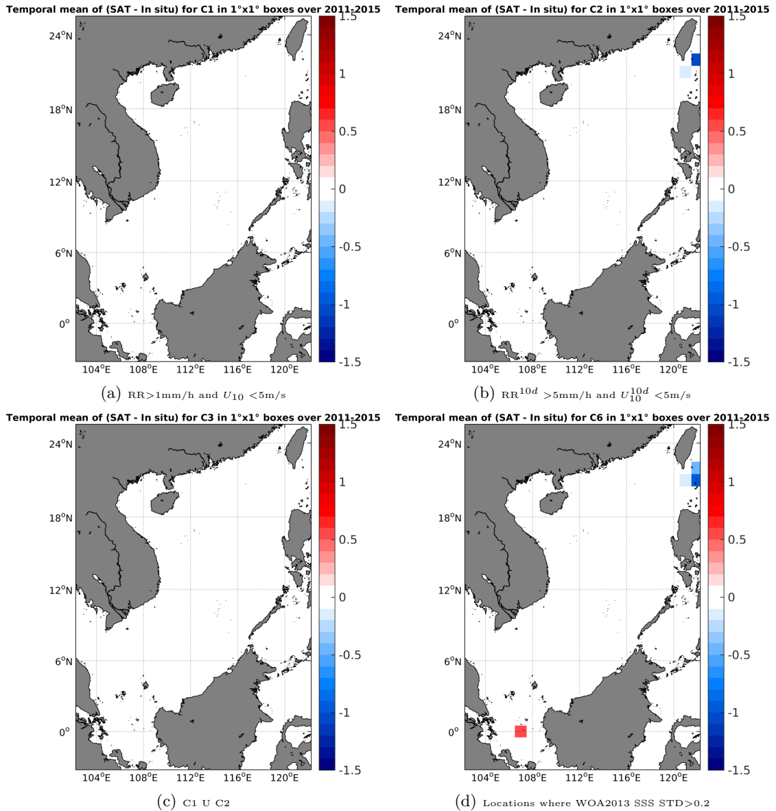
Figure 12: Temporal mean gridded over spatial boxes of size 1°x1° of \Delta SSS (Aquarius-L3-JPL-V4-7DAY-RUNNING - TSG-LEGOS-DM) for 4 different subdatasets corresponding to: RR > 1\text{mm/h} and U_{10} < 5\text{m/s} (a), RR^{10d} > 5\text{mm/h} and U_{10}^{10d} < 5\text{m/s} (b), C1 U C2 (c), Locations where WOA2013 SSS STD > 0.2 (d).
