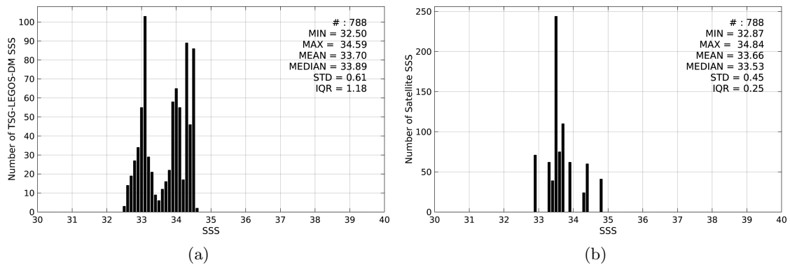
Figure 2: Histograms of SSS from TSG-LEGOS-DM (a) and Aquarius-L3-JPL-V4-7DAY-RUNNING (b) considering all match-up pairs per bins of 0.1 over the South China Sea Pi-MEP region and for the full satellite product period.
