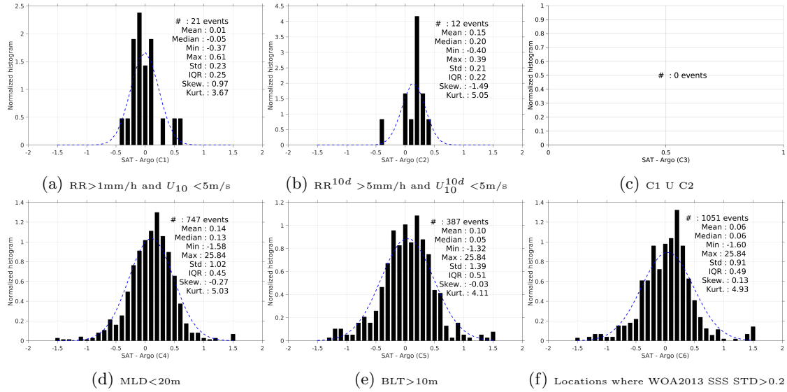
Figure 13: Normalized histogram of \Delta SSS (Aquarius-L3-JPL-V4-7DAY-RUNNING - Argo) for 6 different subdatasets corresponding to: RR > 1mm/h and U_{10} < 5 m/s (a), RR^{10d} > 5 mm/h and U_{10}^{10d} < 5 m/s (b), C1 U C2 (c), MLD < 20m (d), BLT > 10m (e), Locations where WOA2013 SSS STD > 0.2 (f).
