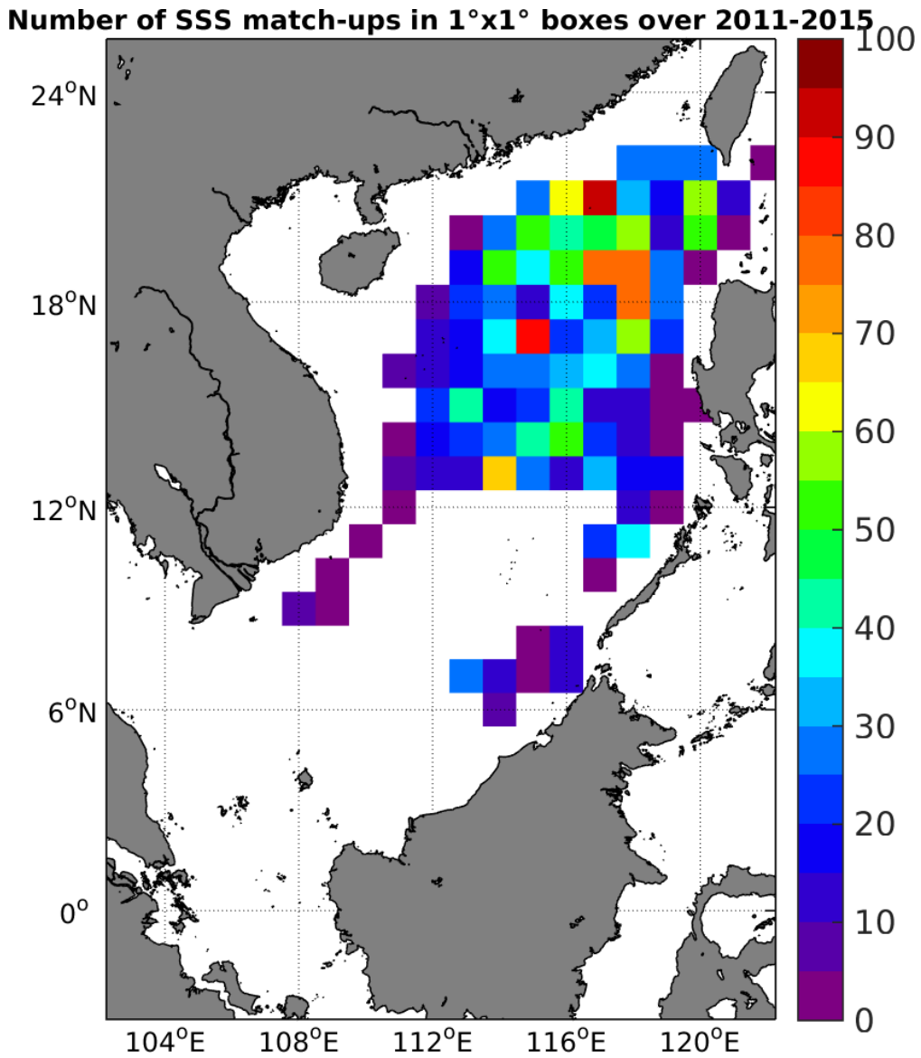
Figure 4: Number of SSS match-ups between Argo SSS and the Aquarius-L3-JPL-V4-7DAY-RUNNING SSS product for the South China Sea Pi-MEP region over 1°x1° boxes and for the full satellite product period.
