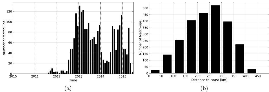
Figure 1: Number of match-ups between Argo and Aquarius-L3-JPL-V4-7DAY-RUNNING SSS as a function of time (a) and as function of the distance to coast (b) over the South China Sea Pi-MEP region and for the full satellite product period.
