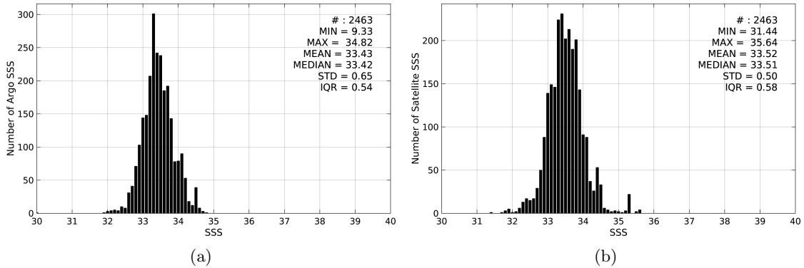
Figure 2: Histograms of SSS from Argo (a) and Aquarius-L3-JPL-V4-7DAY-RUNNING (b) considering all match-up pairs per bins of 0.1 over the South China Sea Pi-MEP region and for the full satellite product period.
