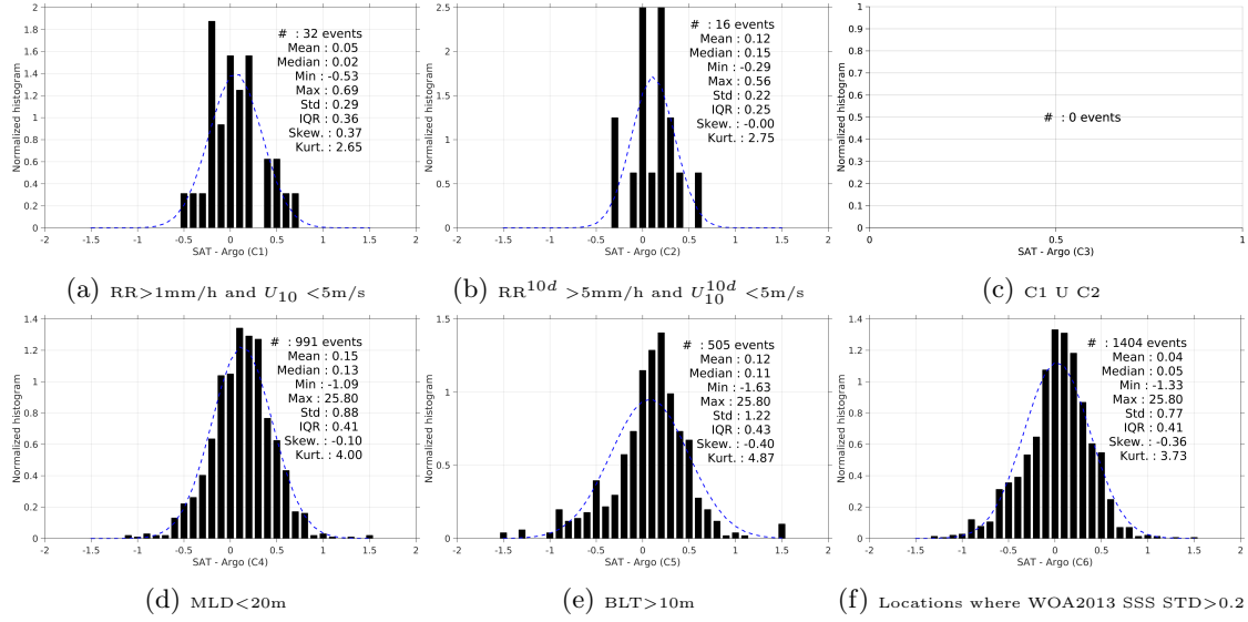
Figure 13: Normalized histogram of \Delta SSS (Aquarius-L3-JPL-V4-MONTHLY - Argo) for 6 different subdatasets corresponding to: RR > 1mm/h and U_{10} < 5 m/s (a), RR 10d > 5mm/h and U_{10}^{10d} < 5 m/s (b), C1 U C2 (c), MLD < 20m (d), BLT > 10m (e), Locations where WOA2013 SSS STD > 0.2 (f).
