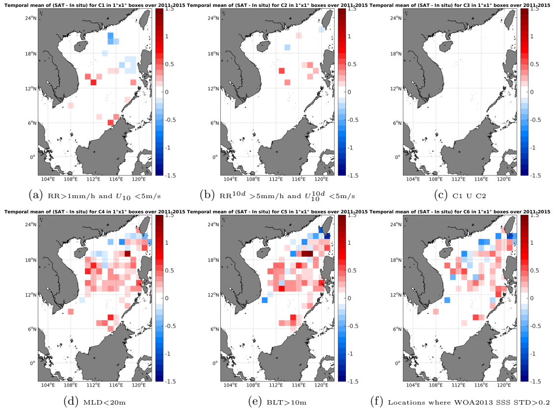
Figure 12: Temporal mean gridded over spatial boxes of size 1^\circ \times 1^\circ of \Delta SSS (Aquarius-L3-JPL-V4-MONTHLY - Argo) for 6 different subdatasets corresponding to: RR > 1\text{mm/h} and U_{10} < 5\text{m/s} (a), RR^{10d} > 5\text{mm/h} and U_{10}^{10d} < 5\text{m/s} (b), C1 U C2 (c), MLD < 20\text{m} (d), BLT > 10\text{m} (e), Locations where WOA2013 SSS STD > 0.2 (f).
