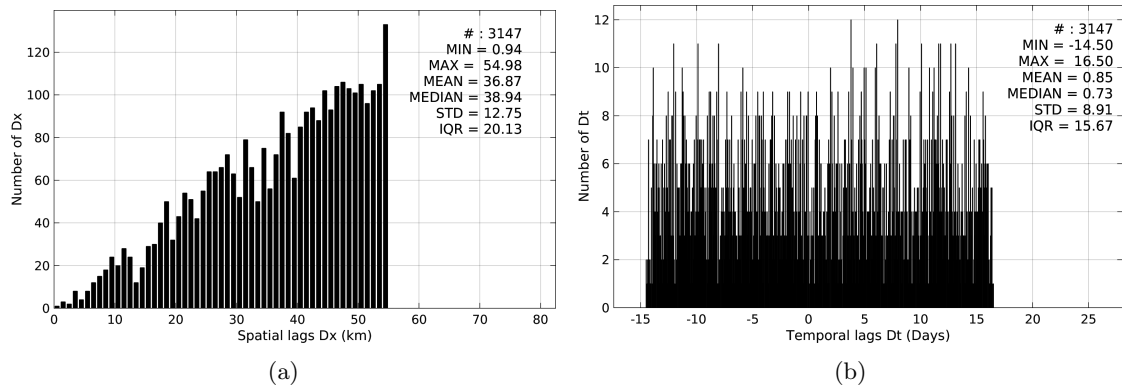
Figure 5: Histograms of the spatial (a) and temporal (b) lags between the time of the Argo measurements and the date of the corresponding Aquarius-L3-JPL-V4-MONTHLY SSS product.
