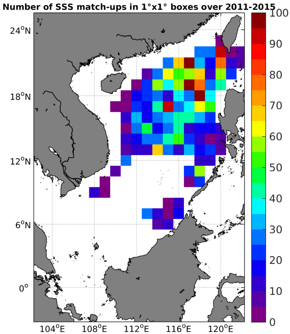
Figure 4: Number of SSS match-ups between Argo SSS and the Aquarius-L3-JPL-V4-MONTHLY SSS product for the South China Sea Pi-MEP region over 1°x1° boxes and for the full satellite product period.
