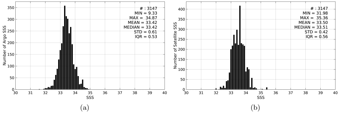
Figure 2: Histograms of SSS from Argo (a) and Aquarius-L3-JPL-V4-MONTHLY (b) considering all match-up pairs per bins of 0.1 over the South China Sea Pi-MEP region and for the full satellite product period.
