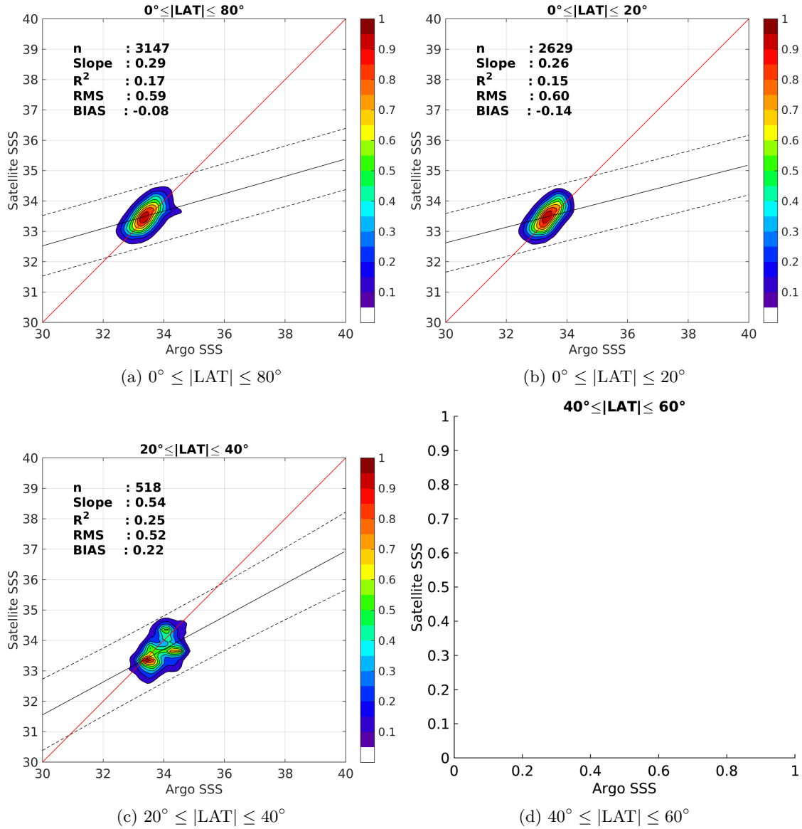
Figure 9: Contour maps of the concentration of Aquarius-L3-JPL-V4-MONTHLY SSS (y-axis) versus Argo SSS (x-axis) at match-up pairs for different latitude bands. For each plot, the red line shows x=y . The black thin and dashed lines indicate a linear fit through the data cloud and the \pm 95\% confidence levels, respectively. The number match-up pairs n , the slope and R^2 coefficient of the linear fit, the root mean square (RMS) and the mean bias between satellite and in situ data are indicated for each latitude band in each plots.
