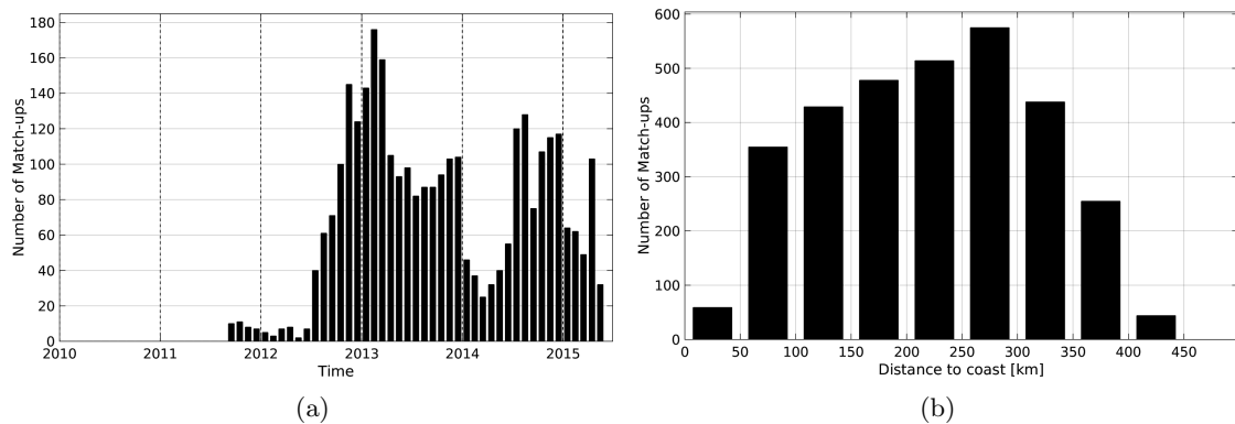
Figure 1: Number of match-ups between Argo and Aquarius-L3-JPL-V4-MONTHLY SSS as a function of time (a) and as function of the distance to coast (b) over the South China Sea Pi-MEP region and for the full satellite product period.
