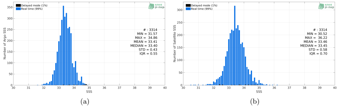
Figure 2: Histograms of SSS from Argo (a) and Aquarius SSS L2-AVERAGED CAP v5 (JPL) (b) considering all match-up pairs per bins of 0.1 over the South China Sea Pi-MEP region and for the full satellite product period.
