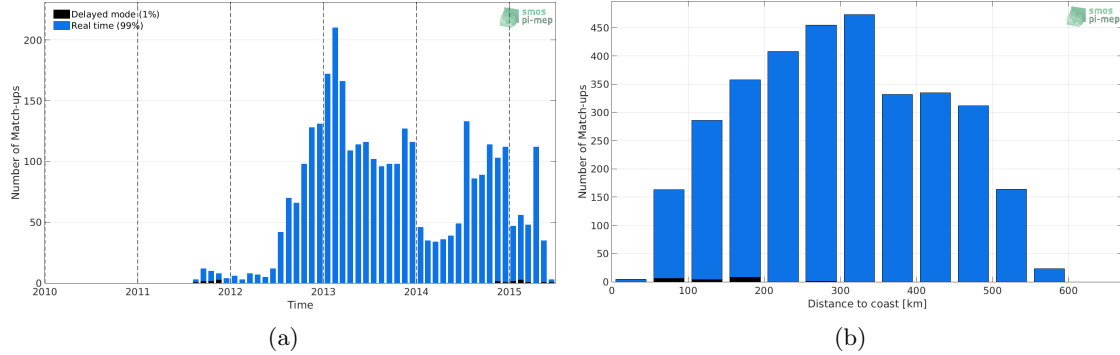
Figure 1: Number of match-ups between Argo and Aquarius SSS L2-AVERAGED CAP v5 (JPL) SSS as a function of time (a) and as function of the distance to coast (b) over the South China Sea Pi-MEP region and for the full satellite product period.
