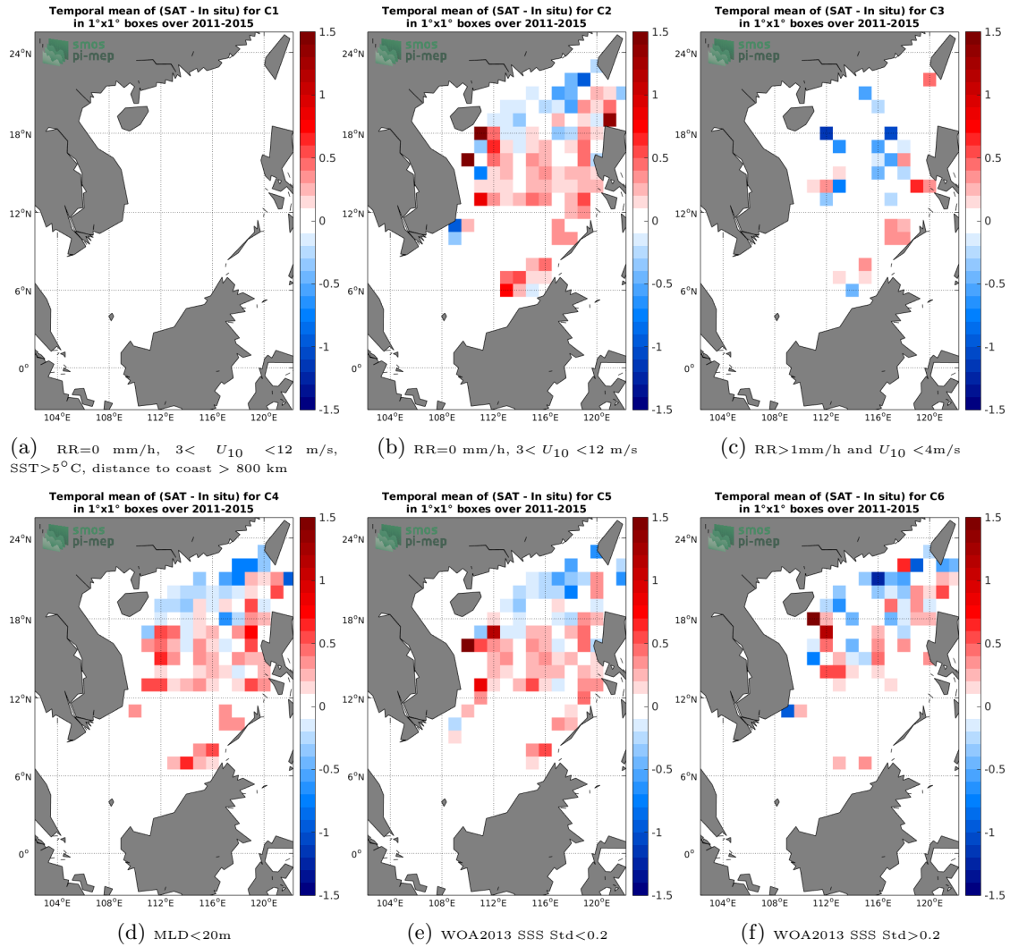
Figure 12: Temporal mean gridded over spatial boxes of size 1^\circ \times 1^\circ of \Delta SSS (Aquarius SSS L2-AVERAGED CAP v5 (JPL) - Argo) for 6 different subdatasets corresponding to: RR=0 mm/h, 3 < U_{10} < 12 m/s, SST > 5°C, distance to coast > 800 km (a), RR=0 mm/h, 3 < U_{10} < 12 m/s (b), RR > 1mm/h and U_{10} < 4 m/s (c), MLD < 20m (d), WOA2013 SSS Std < 0.2 (e), WOA2013 SSS Std > 0.2 (f).
