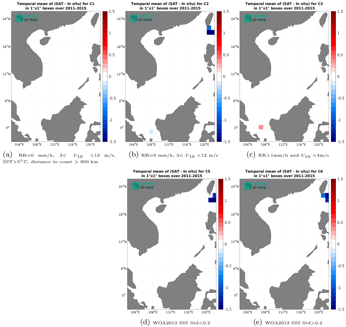
Figure 14: Temporal mean gridded over spatial boxes of size 1^\circ \times 1^\circ of \Delta\text{SSS} (Aquarius SSS L2 OR v5 (NASA-GSFC) - TSG (LEGOS-DM)) for 5 different subdatasets corresponding to: RR=0 mm/h, 3 < U_{10} < 12 m/s, SST > 5^\circ\text{C} , distance to coast > 800 km (a), RR=0 mm/h, 3 < U_{10} < 12 m/s (b), RR > 1 mm/h and U_{10} < 4 m/s (c), WOA2013 SSS Std < 0.2 (d), WOA2013 SSS Std > 0.2 (e).
