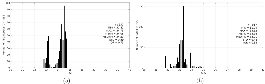
Figure 3: Histograms of SSS from TSG (LEGOS-DM) (a) and Aquarius SSS L2 OR v5 (NASA-GSFC) (b) considering all match-up pairs per bins of 0.1 over the South China Sea Pi-MEP region and for the full satellite product period.
