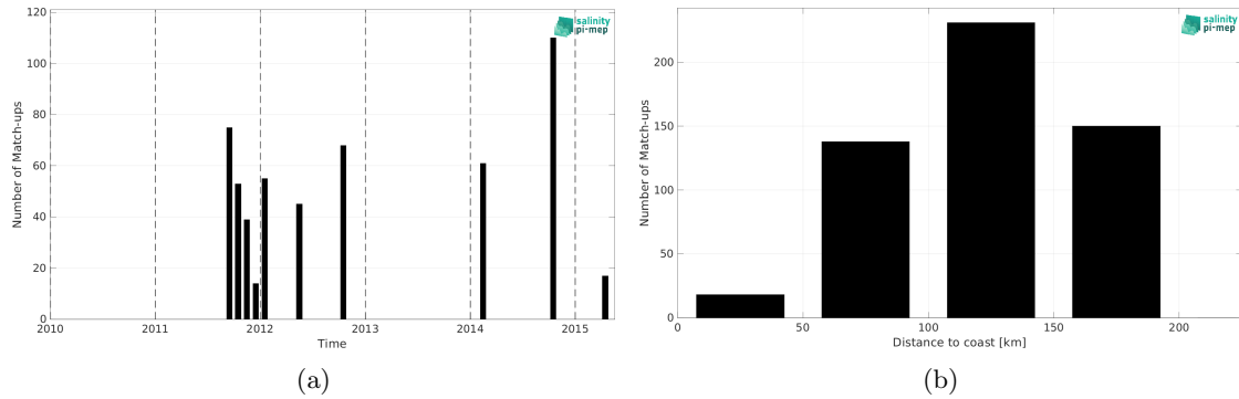
Figure 2: Number of match-ups between TSG (LEGOS-DM) and Aquarius SSS L2 OR v5 (NASA-GSFC) SSS as a function of time (a) and as function of the distance to coast (b) over the South China Sea Pi-MEP region and for the full satellite product period.
