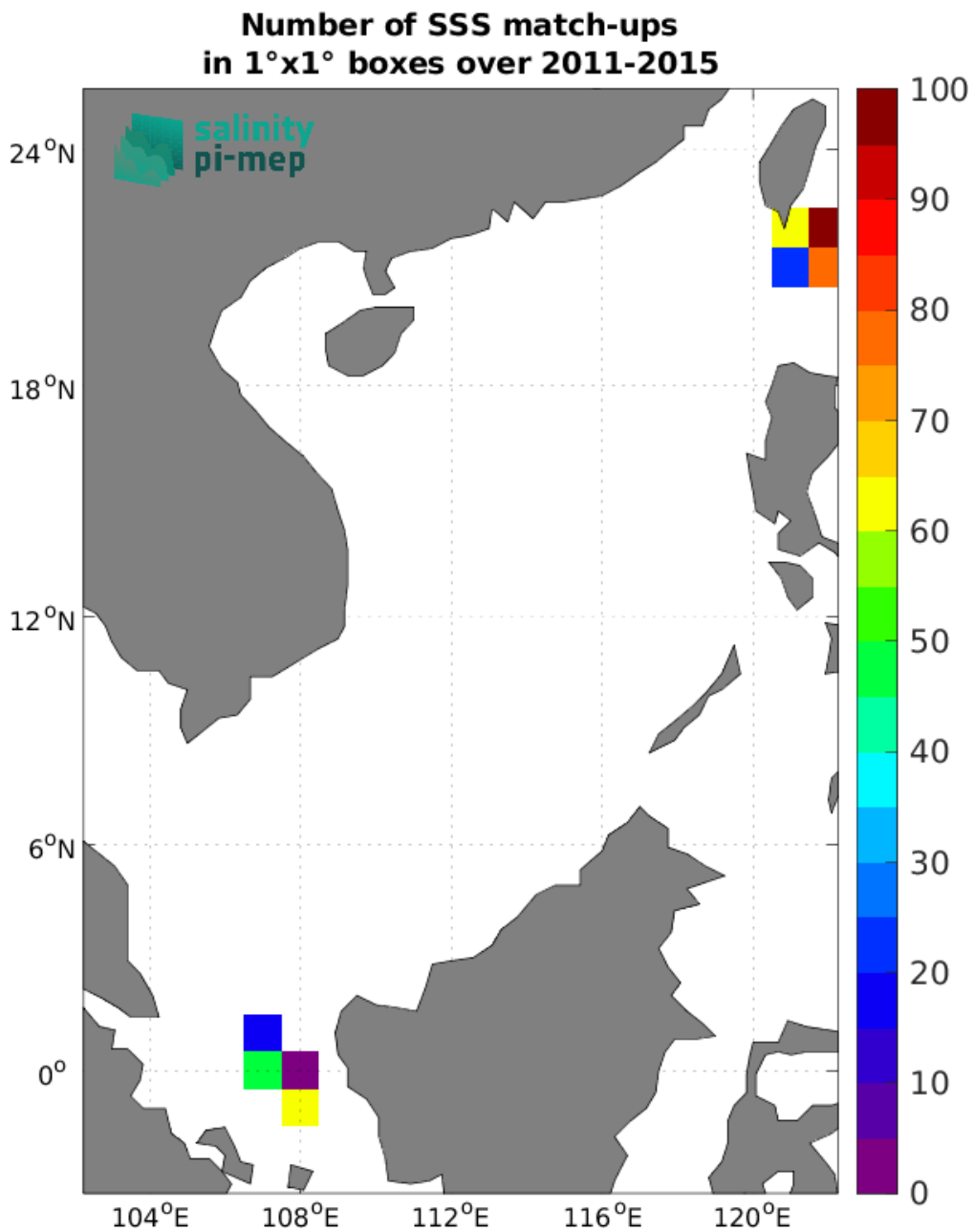
Figure 5: Number of SSS match-ups between TSG (LEGOS-DM) SSS and the Aquarius SSS L2 OR v5 (NASA-GSFC) SSS product for the South China Sea Pi-MEP region over 1^{\circ} \times 1^{\circ} boxes and for the full satellite product period.
