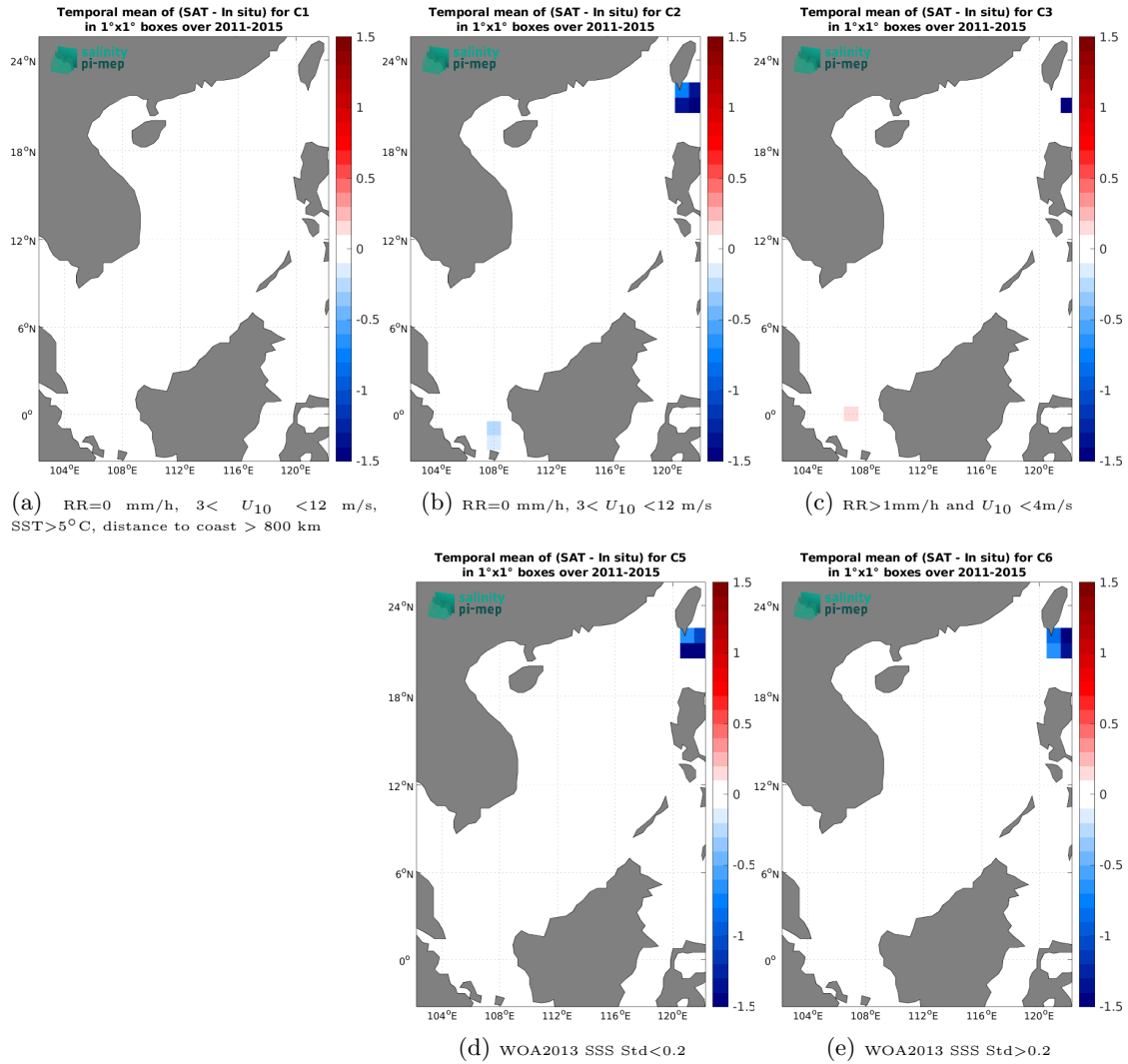
Figure 12: Temporal mean gridded over spatial boxes of size 1^\circ \times 1^\circ of \Delta\text{SSS} (Aquarius SSS L2 OR v5 (NASA-GSFC) - TSG (LEGOS-DM)) for 5 different subdatasets corresponding to: RR=0 mm/h, 3 < U_{10} < 12 m/s, SST > 5^\circ\text{C} , distance to coast > 800 km (a), RR=0 mm/h, 3 < U_{10} < 12 m/s (b), RR > 1 mm/h and U_{10} < 4 m/s (c), WOA2013 SSS Std < 0.2 (d), WOA2013 SSS Std > 0.2 (e).
