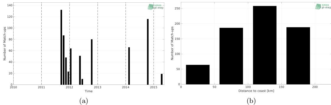
Figure 1: Number of match-ups between TSG (LEGOS-DM) and Aquarius SSS L2 OR v5 (NASA-GSFC) SSS as a function of time (a) and as function of the distance to coast (b) over the South China Sea Pi-MEP region and for the full satellite product period.
