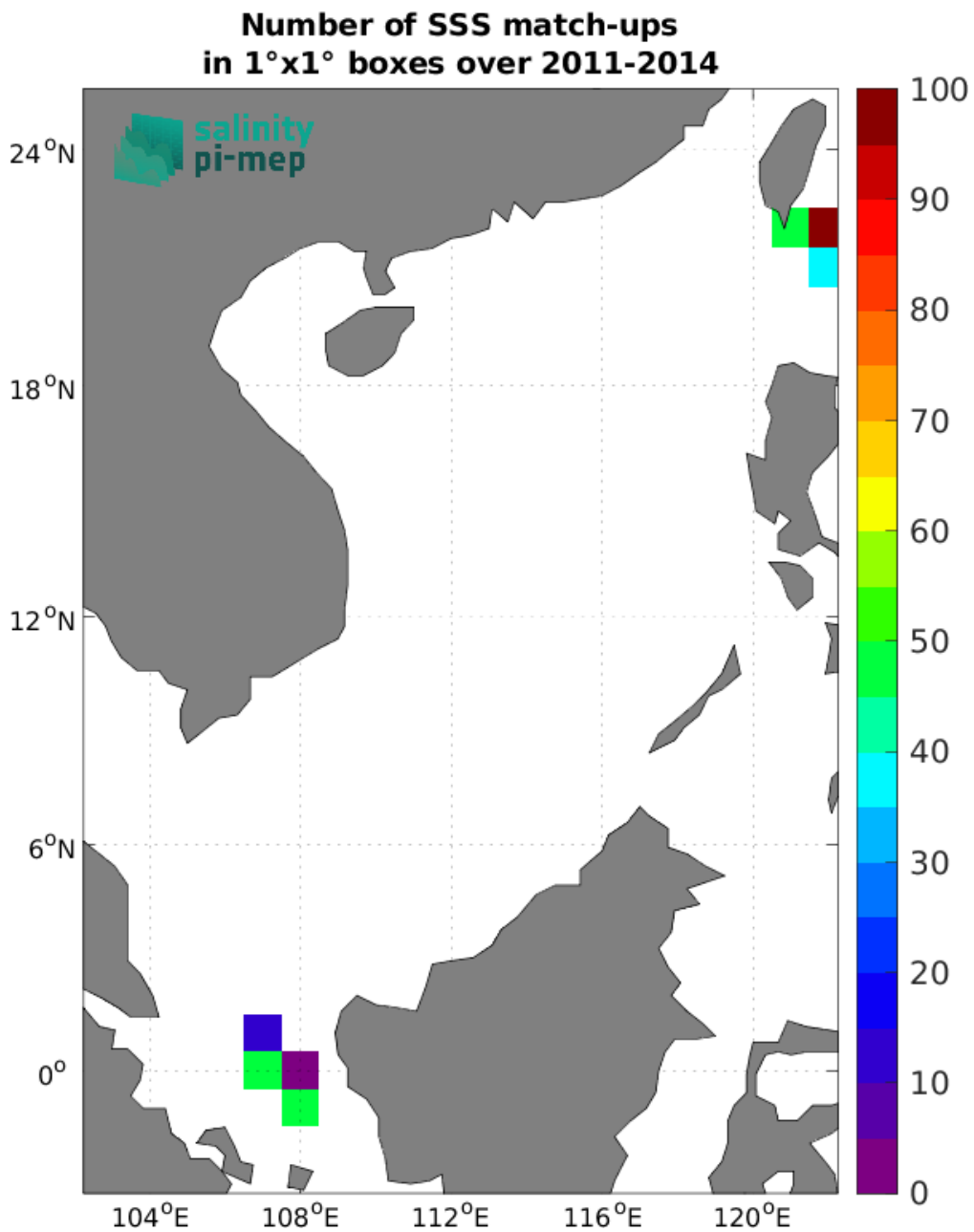
Figure 5: Number of SSS match-ups between TSG (LEGOS-DM) SSS and the Aquarius SSS L2 CAP v5 (JPL) SSS product for the South China Sea Pi-MEP region over 1°×1° boxes and for the full satellite product period.
