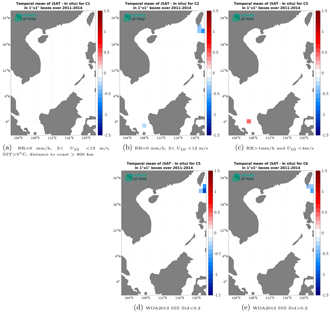
Figure 14: Temporal mean gridded over spatial boxes of size 1°x1° of \Delta SSS (Aquarius SSS L2 CAP v5 (JPL) - TSG (LEGOS-DM)) for 5 different subdatasets corresponding to:RR=0 mm/h, 3 < U_{10} < 12 m/s, SST>5°C, distance to coast > 800 km (a), RR=0 mm/h, 3 < U_{10} < 12 m/s (b), RR>1mm/h and U_{10} < 4 m/s (c), WOA2013 SSS Std<0.2 (d), WOA2013 SSS Std>0.2 (e).
