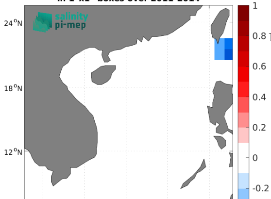
Temporal mean of (Sat - TSG (LEGOS-DM)) in 1°x1° boxes over 2011-2014
