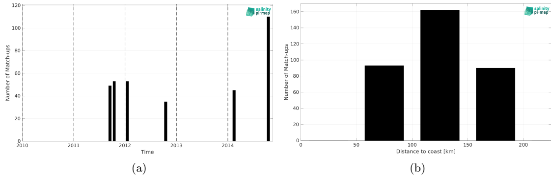
Figure 2: Number of match-ups between TSG (LEGOS-DM) and Aquarius SSS L2 CAP v5 (JPL) SSS as a function of time (a) and as function of the distance to coast (b) over the South China Sea Pi-MEP region and for the full satellite product period.
