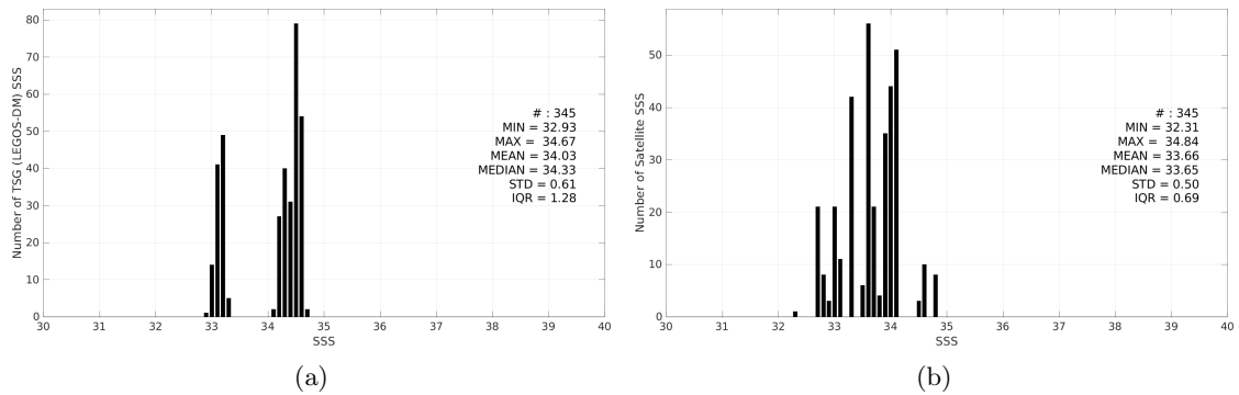
Figure 3: Histograms of SSS from TSG (LEGOS-DM) (a) and Aquarius SSS L2 CAP v5 (JPL) (b) considering all match-up pairs per bins of 0.1 over the South China Sea Pi-MEP region and for the full satellite product period.
