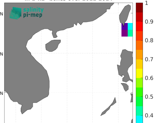
Temporal STD of (Sat - TSG (LEGOS-DM)) in 1°x1° boxes over 2011-2014
