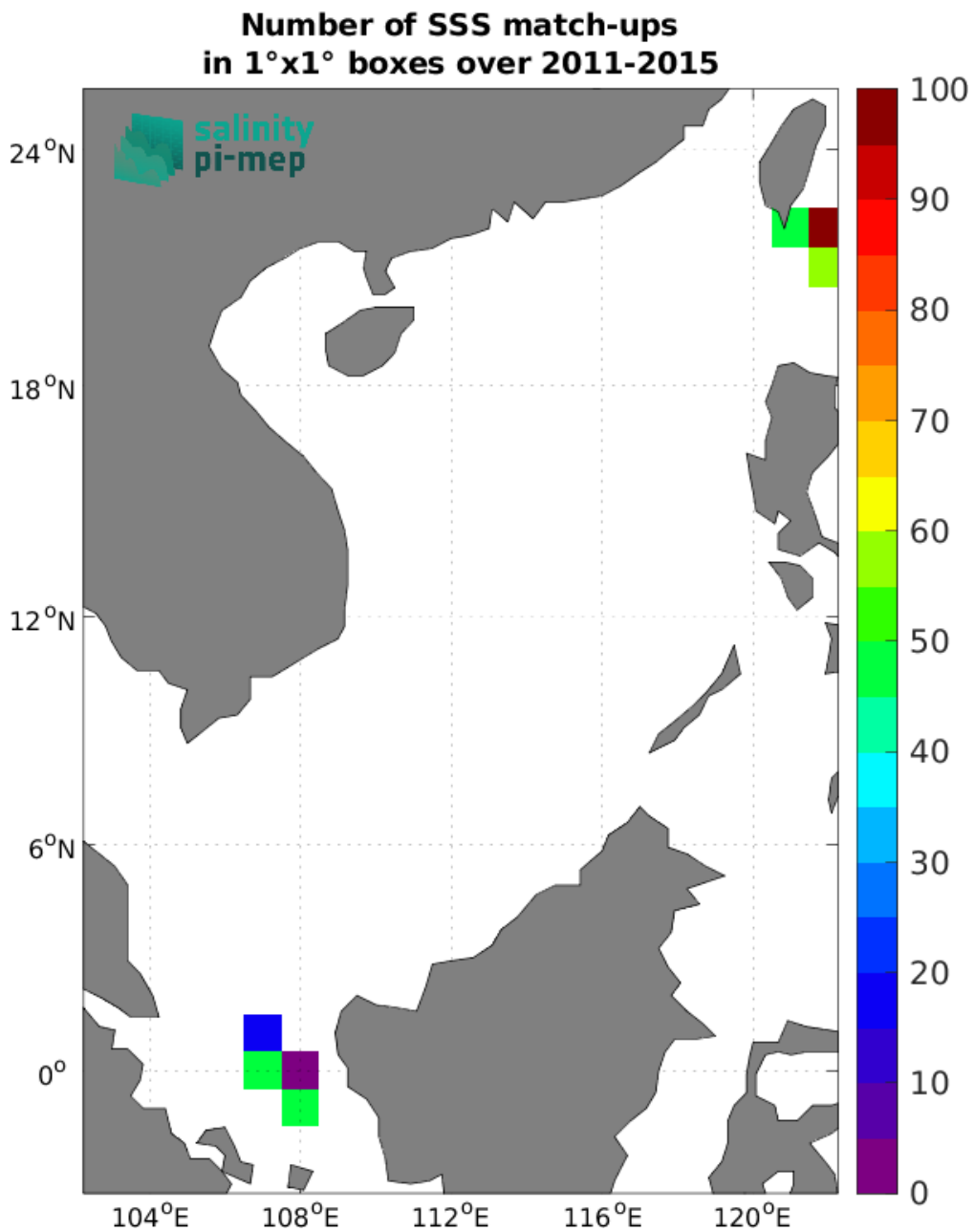
Figure 4: Number of SSS match-ups between TSG (LEGOS-DM) SSS and the Aquarius SSS L2 CAP v5 (JPL) SSS product for the South China Sea Pi-MEP region over 1^\circ \times 1^\circ boxes and for the full satellite product period.
