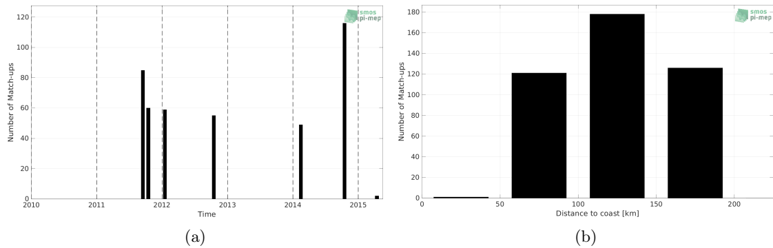
Figure 1: Number of match-ups between TSG (LEGOS-DM) and Aquarius SSS L2 CAP v5 (JPL) SSS as a function of time (a) and as function of the distance to coast (b) over the South China Sea Pi-MEP region and for the full satellite product period.
