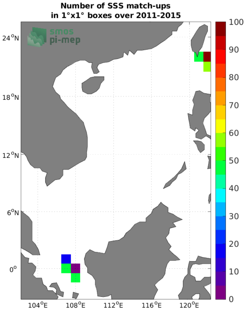
Figure 4: Number of SSS match-ups between TSG (LEGOS-DM) SSS and the Aquarius SSS L2 CAP v5 (JPL) SSS product for the South China Sea Pi-MEP region over 1°×1° boxes and for the full satellite product period.
