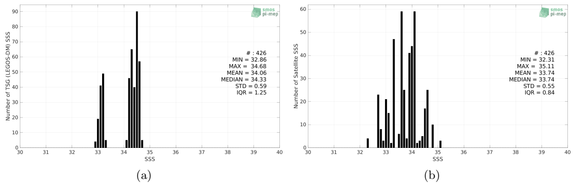
Figure 2: Histograms of SSS from TSG (LEGOS-DM) (a) and Aquarius SSS L2 CAP v5 (JPL) (b) considering all match-up pairs per bins of 0.1 over the South China Sea Pi-MEP region and for the full satellite product period.
