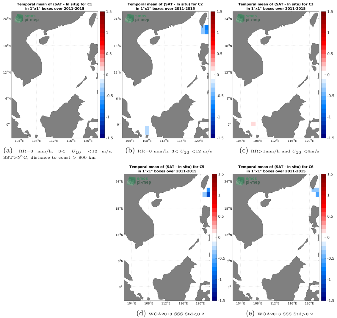
Figure 12: Temporal mean gridded over spatial boxes of size 1^\circ \times 1^\circ of \Delta SSS (Aquarius SSS L2 CAP v5 (JPL) - TSG (LEGOS-DM)) for 5 different subdatasets corresponding to: RR=0 mm/h, 3 < U_{10} < 12 m/s, SST > 5°C, distance to coast > 800 km (a), RR=0 mm/h, 3 < U_{10} < 12 m/s (b), RR > 1mm/h and U_{10} < 4 m/s (c), WOA2013 SSS Std < 0.2 (d), WOA2013 SSS Std > 0.2 (e).
