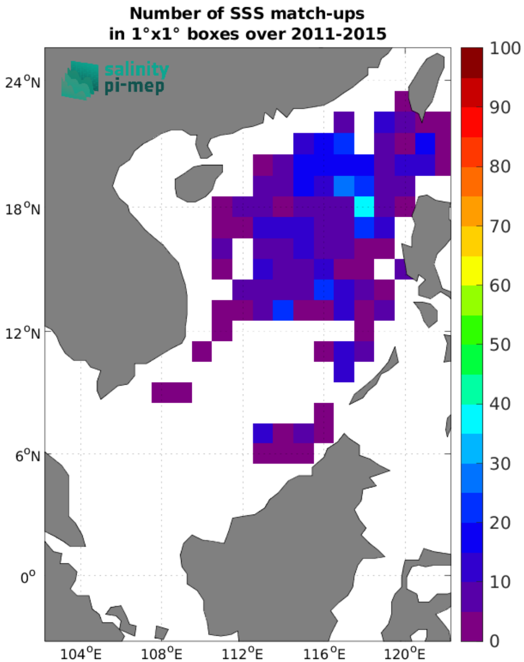
Figure 4: Number of SSS match-ups between Argo SSS and the Aquarius SSS L2 CAP v5 (JPL) SSS product for the South China Sea Pi-MEP region over 1^\circ \times 1^\circ boxes and for the full satellite product period.
